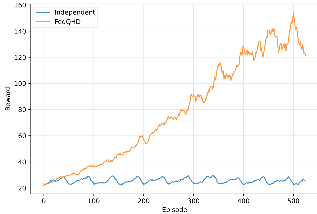
N = 50 clients
