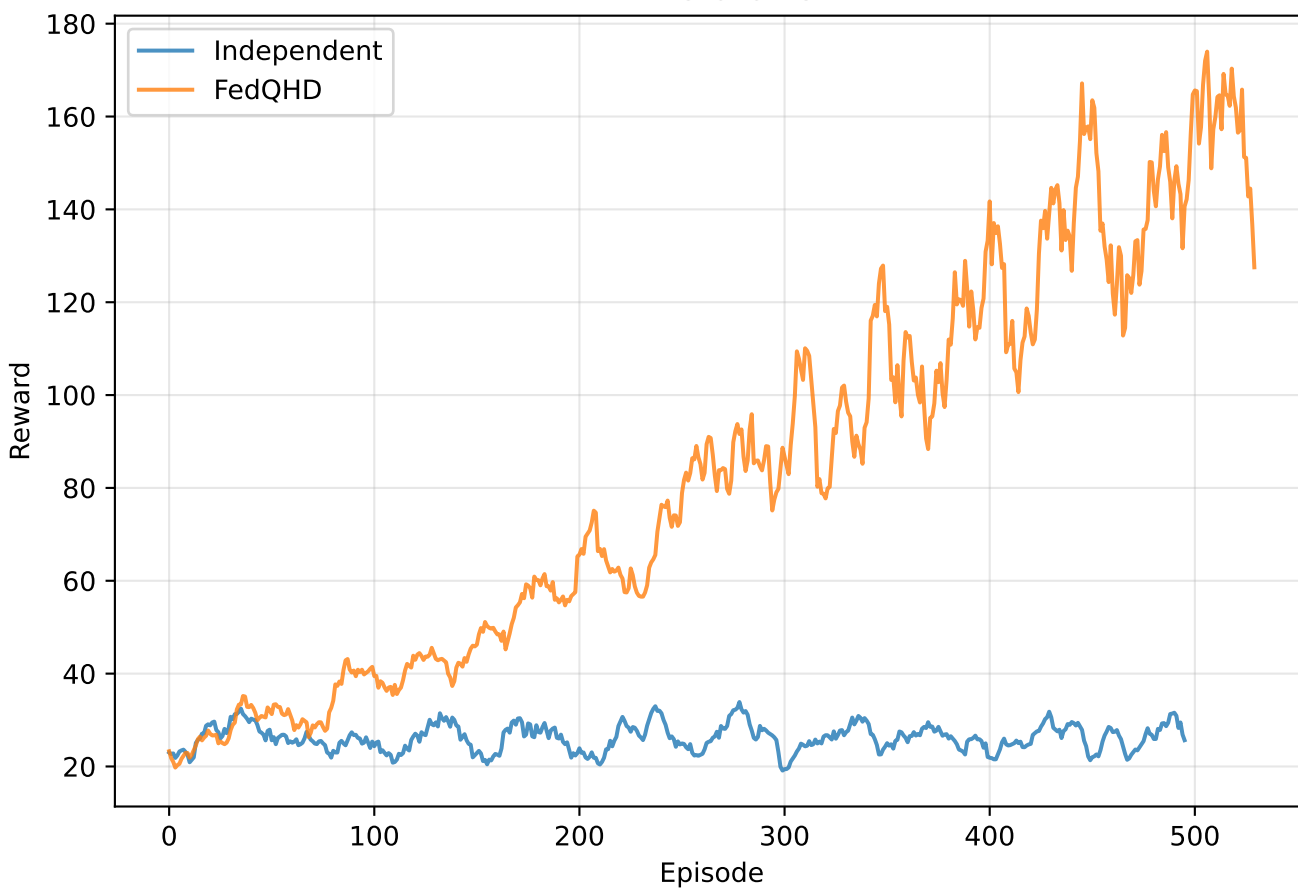
N = 20 clients
