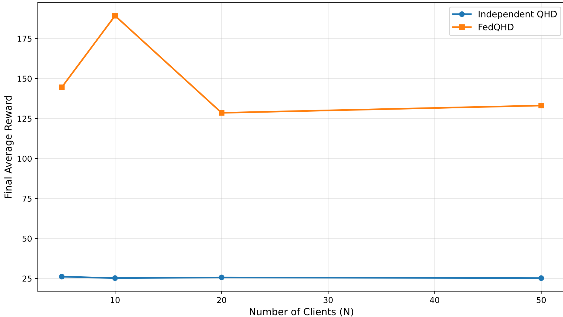
Scalability: Performance vs. Number of Clients
