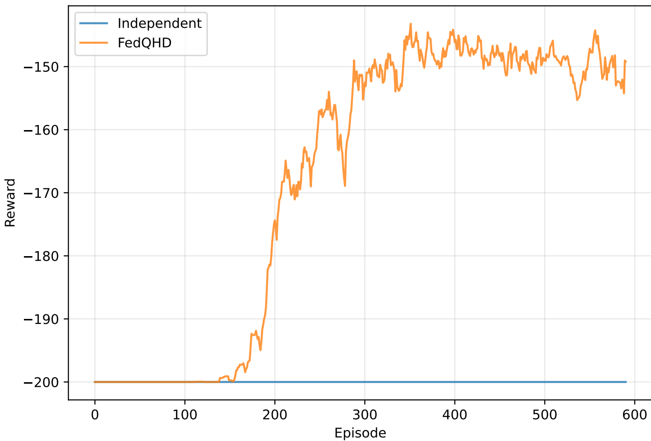
N = 20 clients
