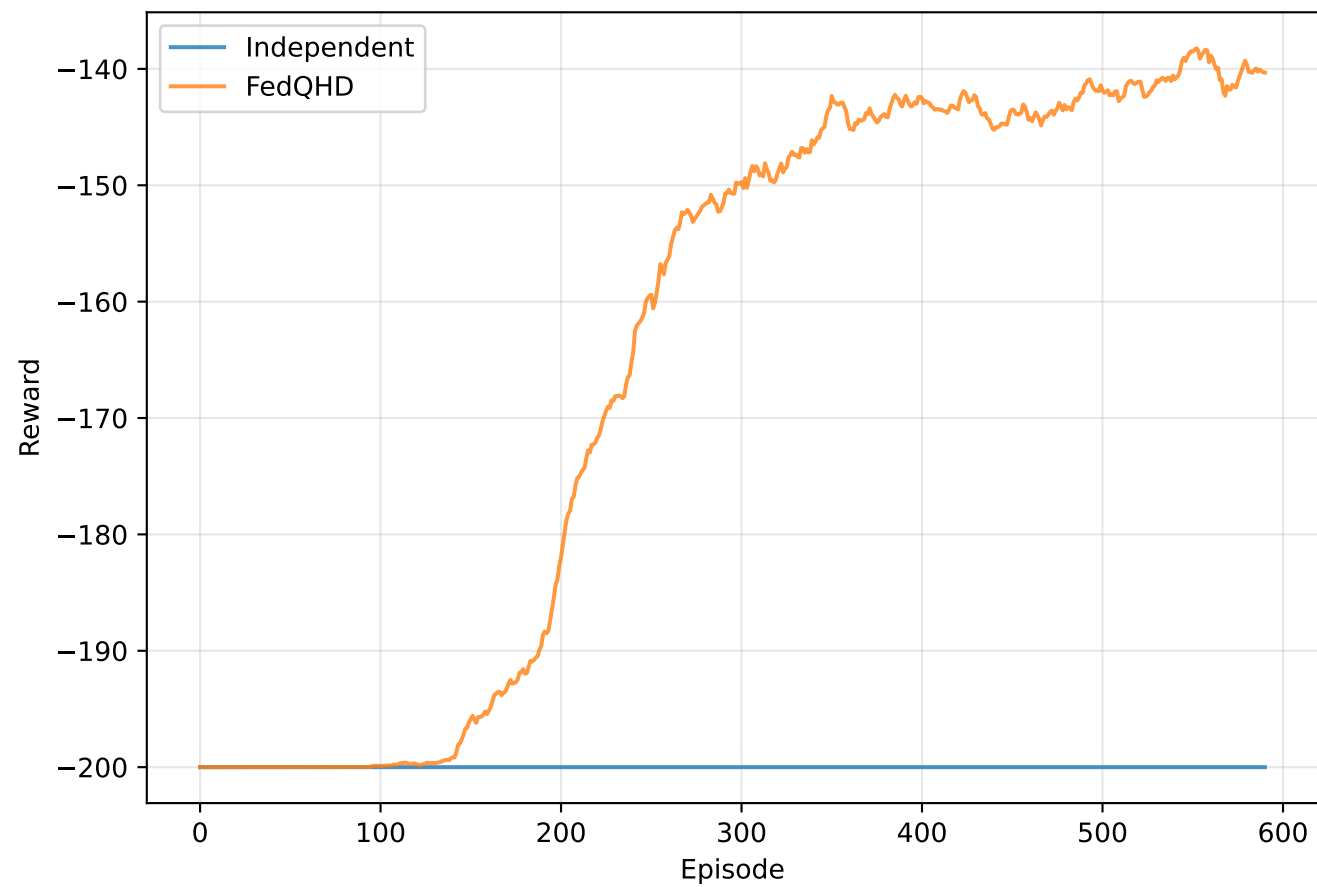
N = 50 clients
