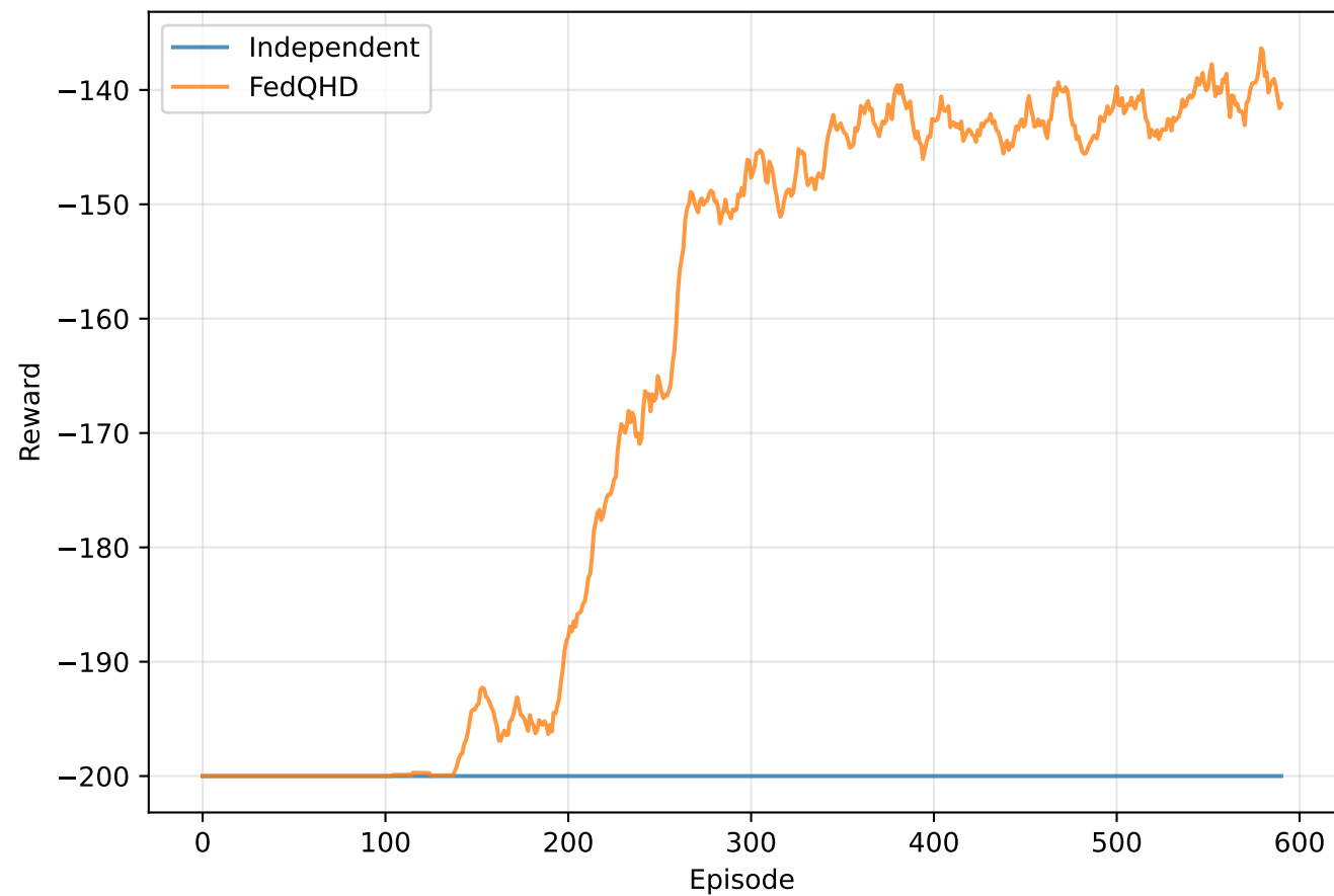
N = 50 clients
