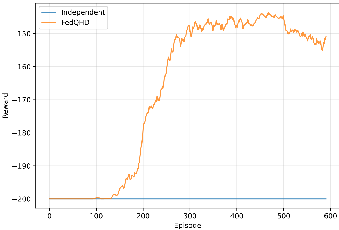
N = 20 clients
