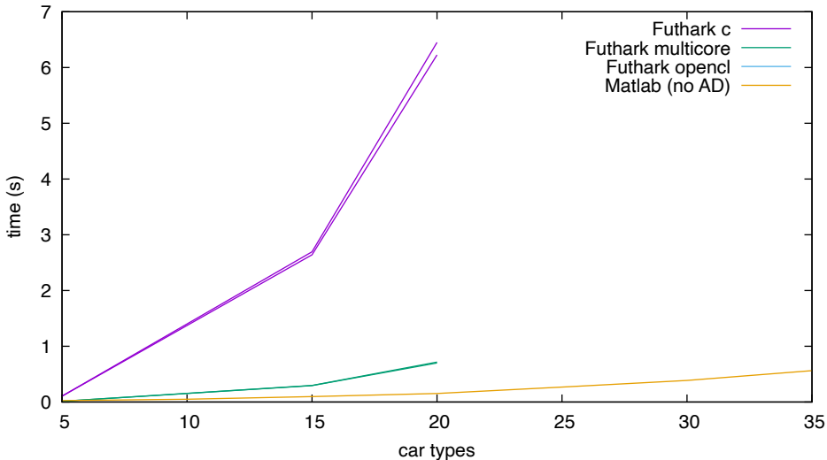
Time (4 households, maxage 25 years) with AD and Newton's method
