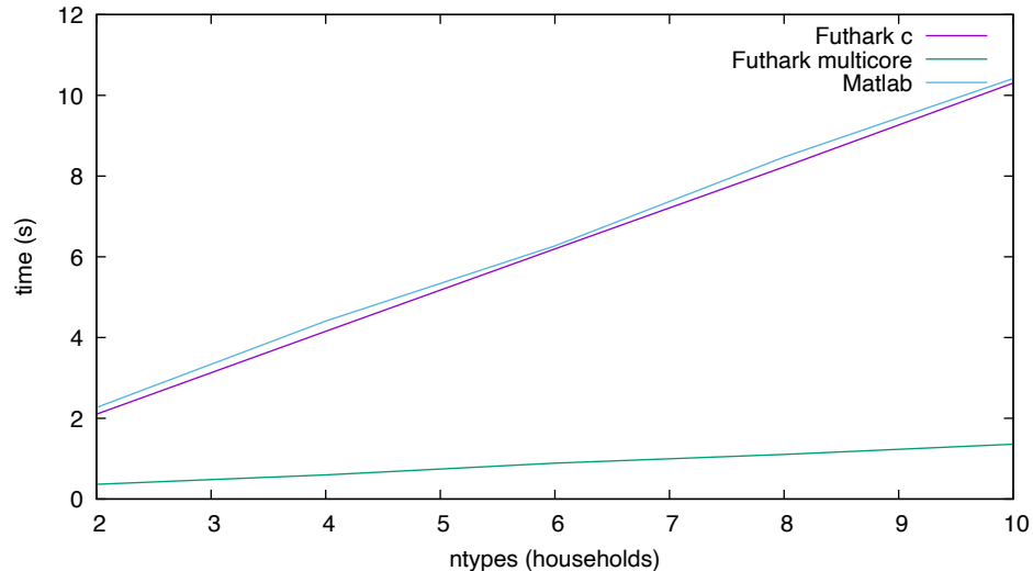
Time (35 car types, maxage 25 years)
