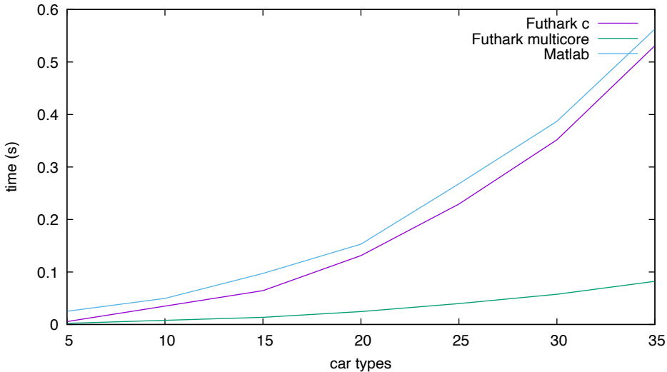
Time (4 households, maxage 25 years) with Newton's method
