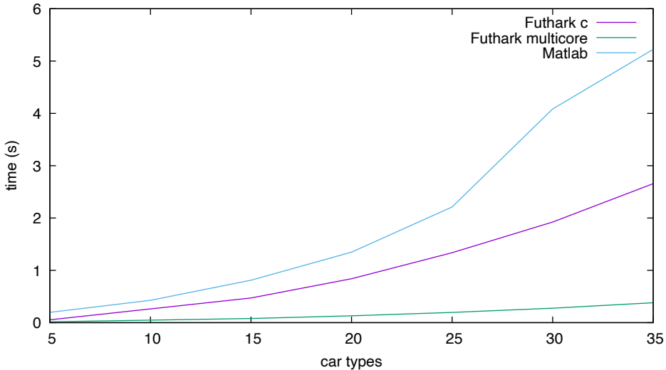
Time (4 households, maxage 20 years)
