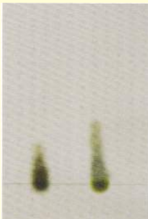
TLC plate of Jaborandi Q in fluorescent light after test
