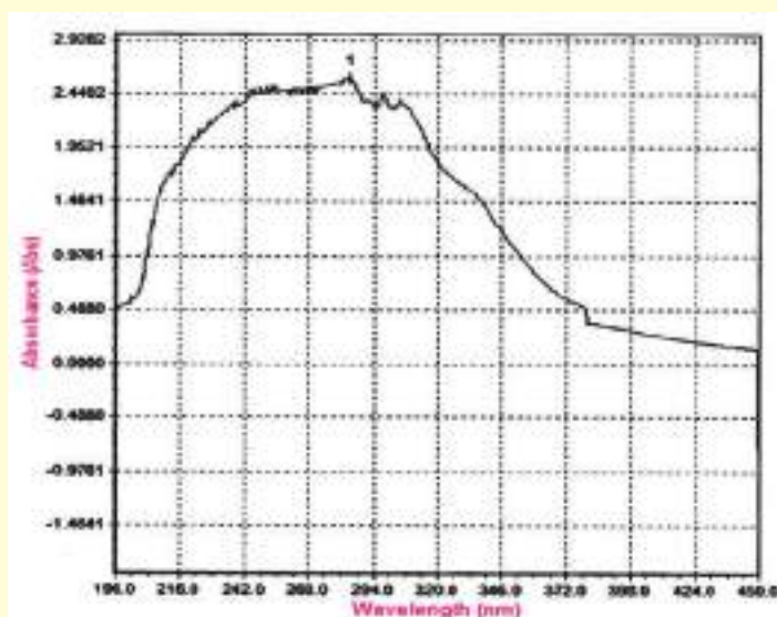
UV Spectro graph of sample of Rauvolfia Serp. Q (PHBL)
