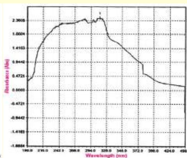
UV Spectro graph of sample of Rauvolfia Serp. Q (another leading company)
