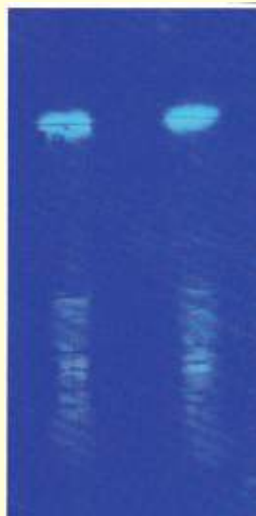
TLC plate of Rauvolfia Serp. Q under long wave UV light.
