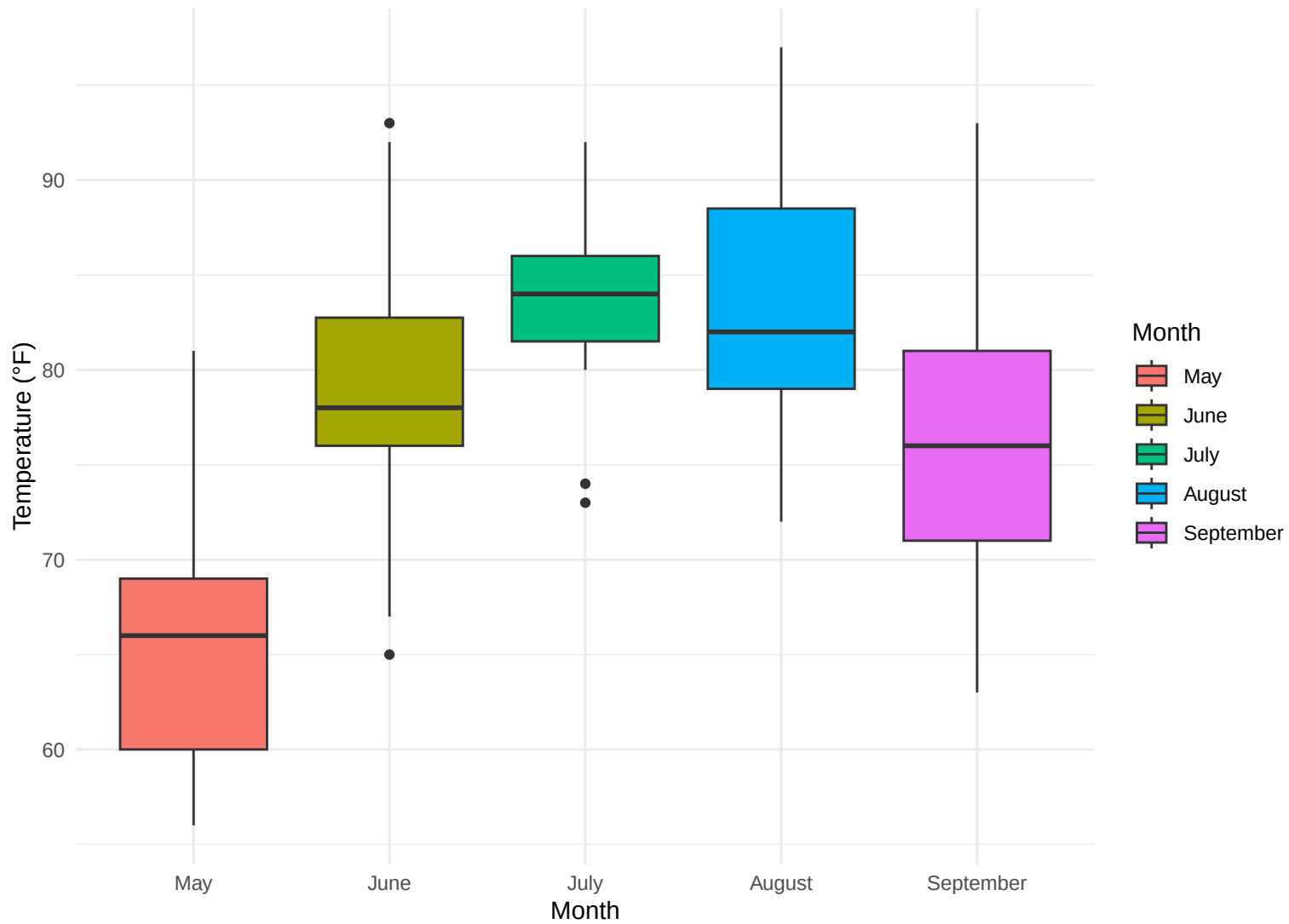
Temperature Distribution by Month
