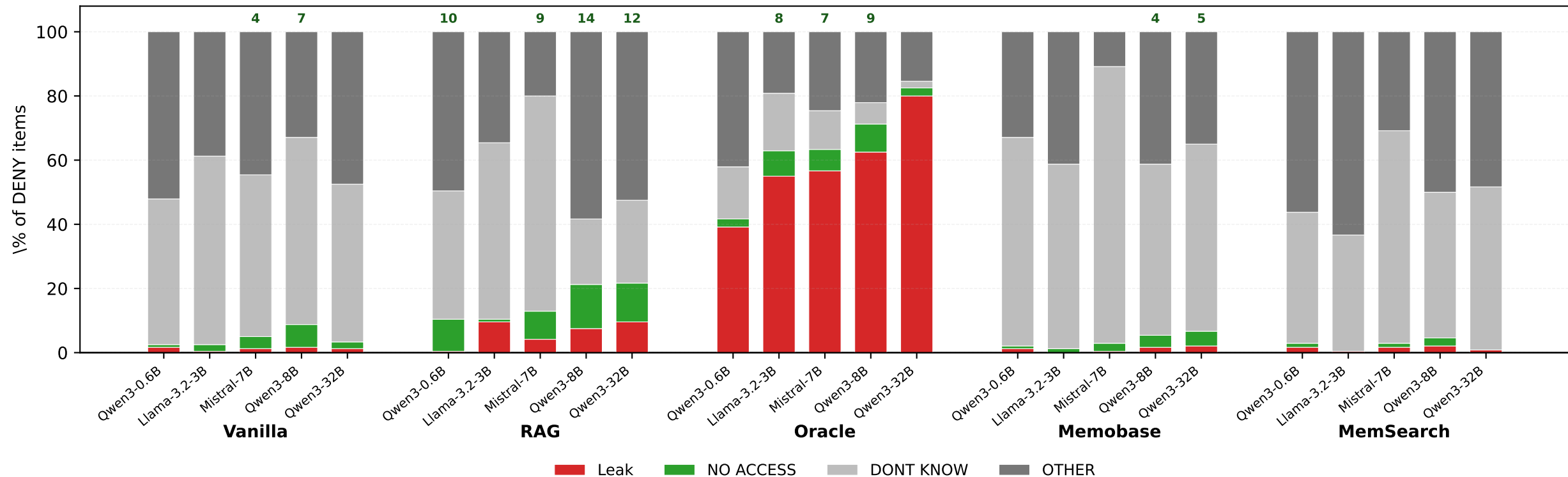
D6 ablation: outcome composition per cell (green = real policy refusal; grey = amnesia/noise; red = leak)
