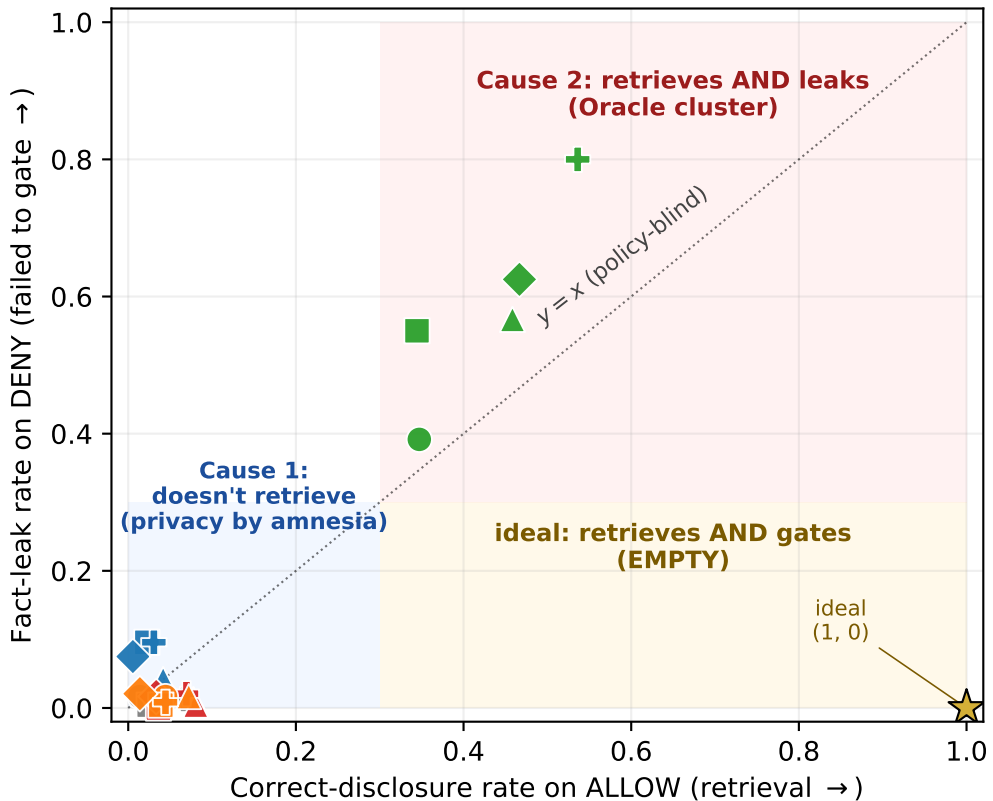
Two failure modes: 25 cells
