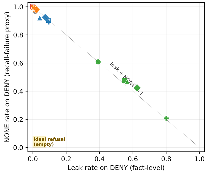
(b) Failure-mode dialectic on DENY
