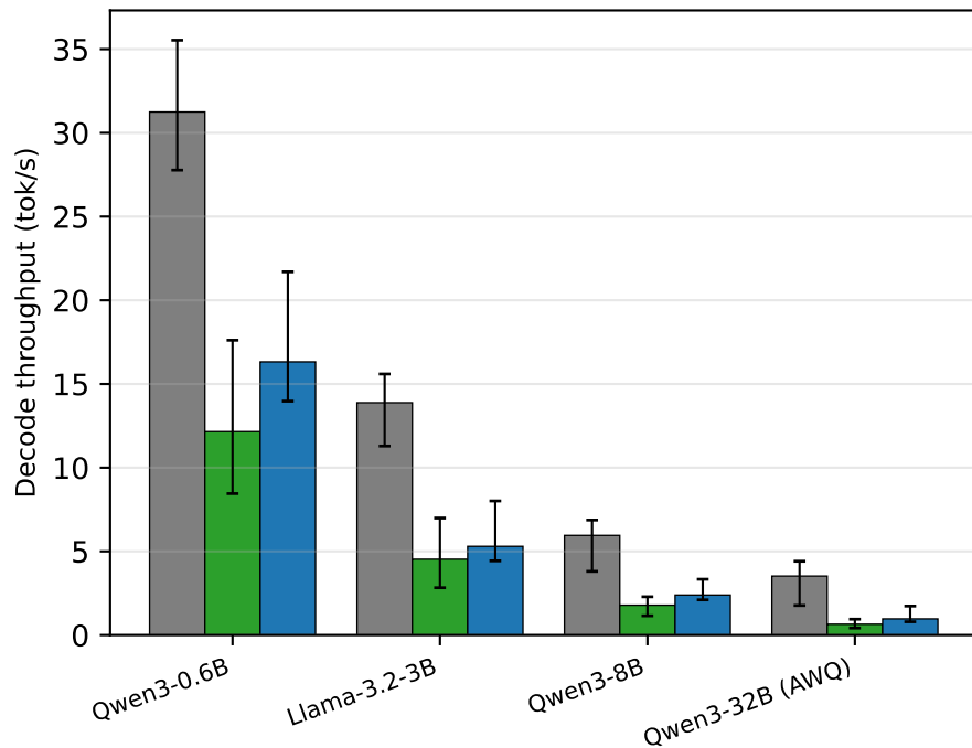
(b) Generation throughput by model
