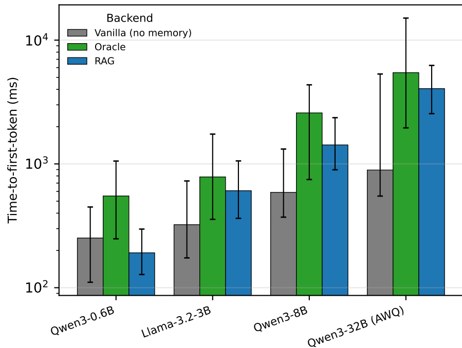
(a) TTFT by model tier
