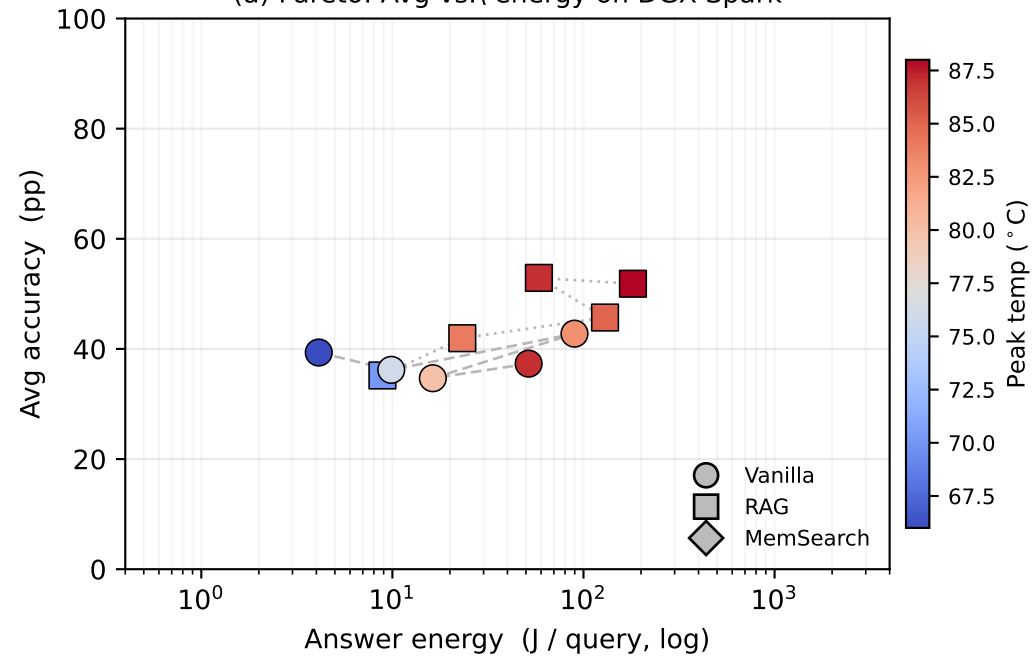
(a) Pareto: Avg vs.\ energy on DGX Spark
