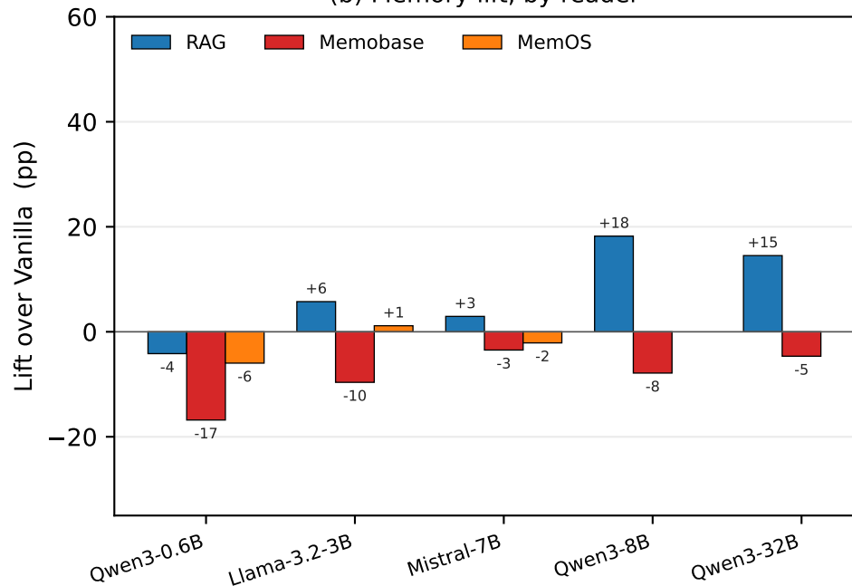
(b) Memory lift, by reader
