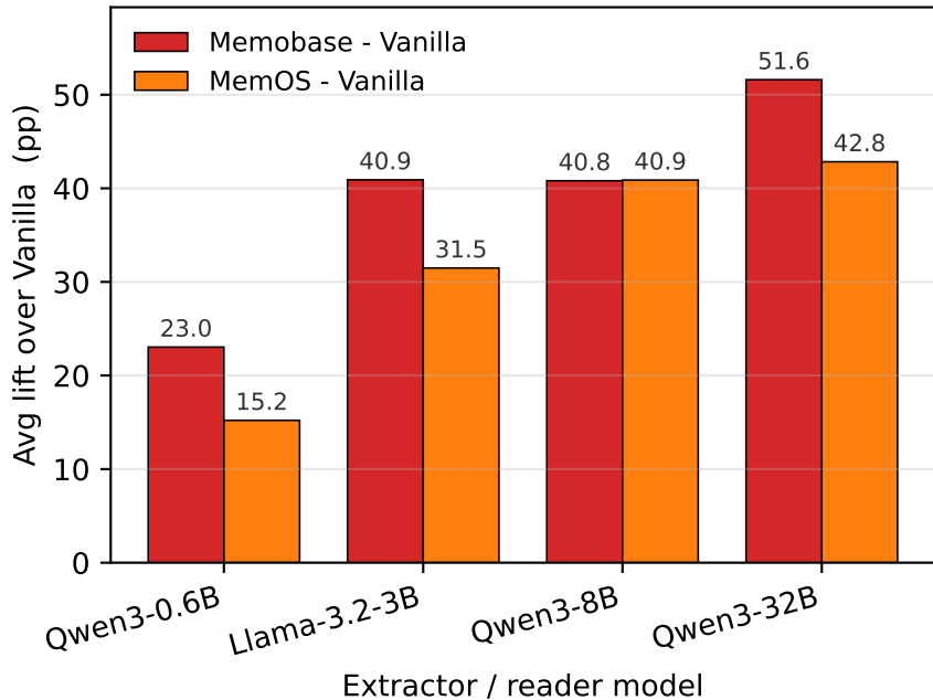
(b) Memory lift grows with model size
