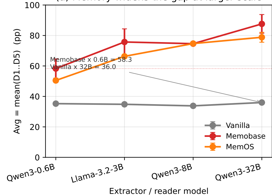
(a) Memory widens the gap at larger scale
