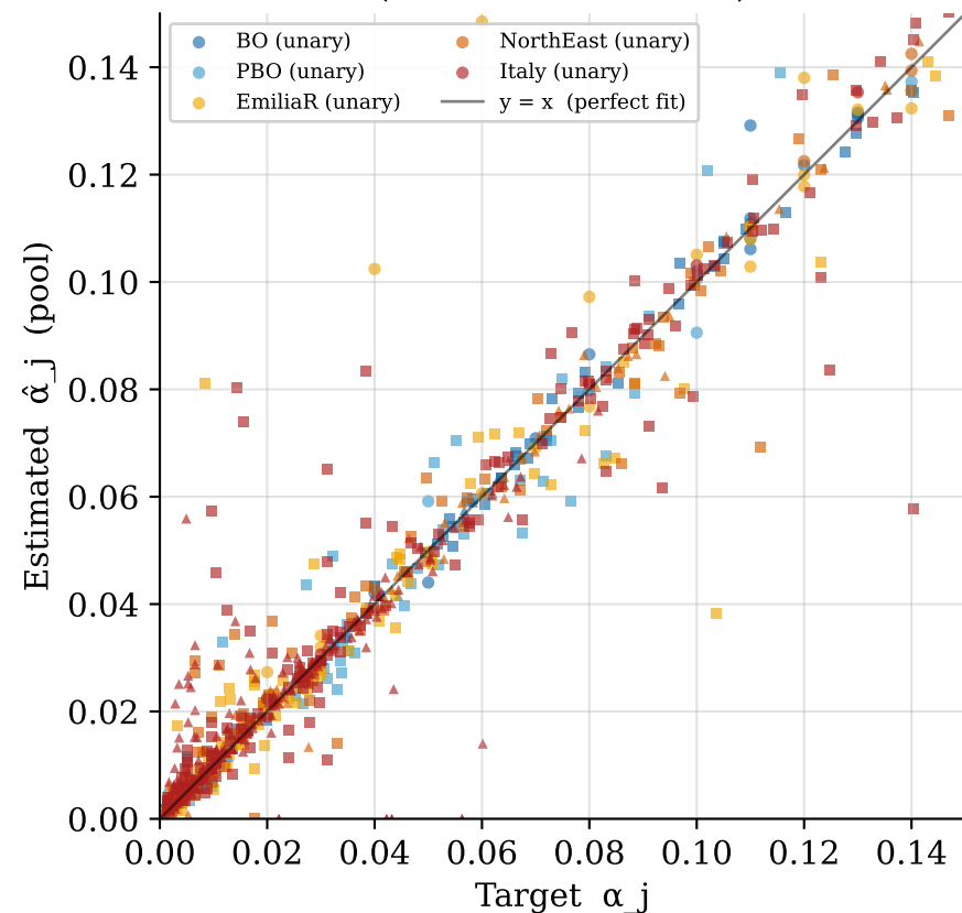
Constraint frequencies: target vs. estimate (zoomed \alpha < 0.15 )
