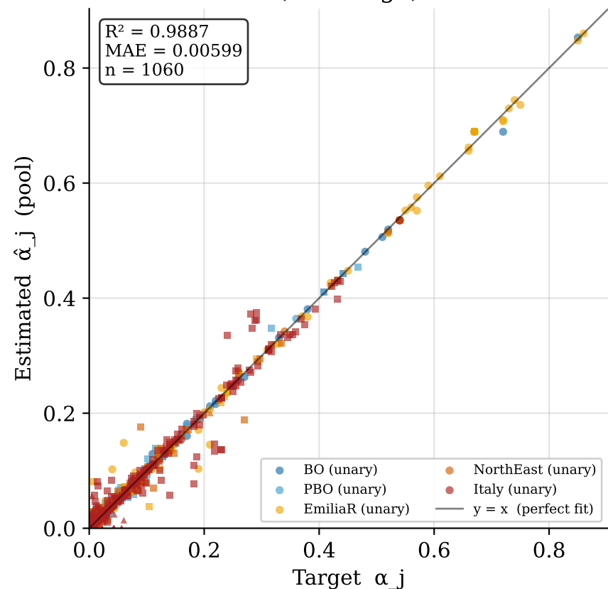
Constraint frequencies: target vs. estimate (full range)
