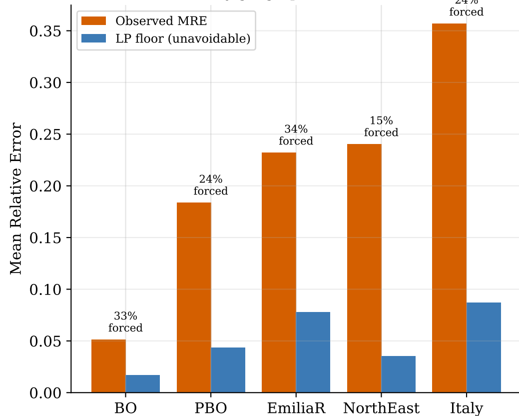
Observed error vs. rigorous lower bound by geographic source
