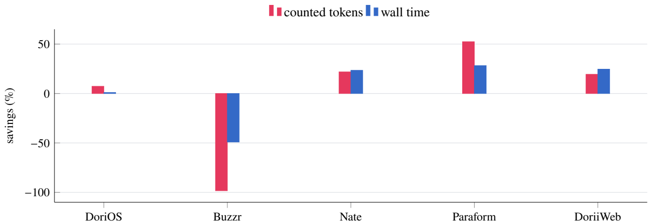
Figure 4: Canonical writable product workflows. Each condition passed its automated acceptance contract; Buzzr nevertheless regressed substantially.
