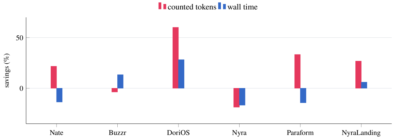
Figure 3: Revision-matched read-only pilot. Positive values favor Memi. The negative Nyra result is retained.
