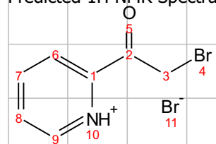
Predicted 1 H NMR Spectrum
