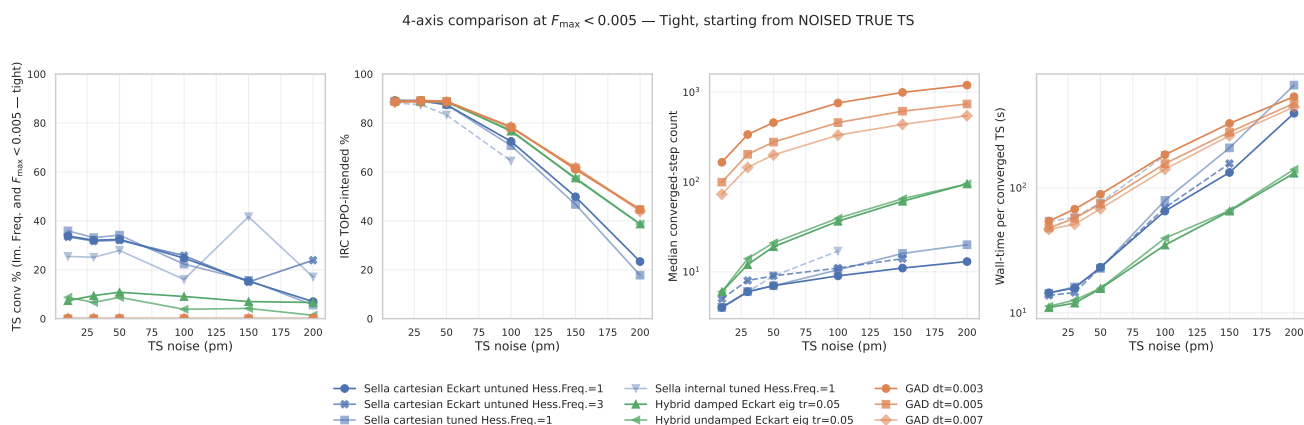
Figure 6: 4-axis @ F_{\max} < 0.005 (tight). Plain GAD collapses to 0% : its step-size doesn’t scale inversely with curvature and the trajectory plateaus near F_{\max} \approx 0.01 . Hybrid retains 7–11% across noise (Newton landing). Sella drops smoothly from 34% to 7%. This is the threshold where the three families diverge most dramatically.
