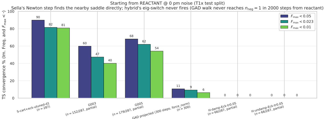
Figure 2: Starting from REACTANT @ 0 pm noise. TS conv % at three F_{\text{max}} thresholds (0.05, 0.023 [Gaussian], 0.01 [project canonical]). Sella (cart+Eckart untuned d=1) lands ~81% of saddles even starting from the reactant — Newton step climbs to the closest saddle direction within ~20 iterations. Plain GAD (dt=0.003, dt=0.005) needs >1000 steps to walk reactant→saddle and partial-run statistics ( n = 152/287, 179/287 ) show 40–54% conv at the project threshold. The 300-step GAD-projected cell (force-norm criterion, no fmax in the trajectory schema) illustrates the step-budget collapse: only 6% converge with a 300-step cap. Hybrid damped/undamped from reactant: 0% conv at all thresholds ( n = 51 each) — a clear mechanistic finding (see following paragraph). Source: reactant_0pm_2026_05_16.csv .
