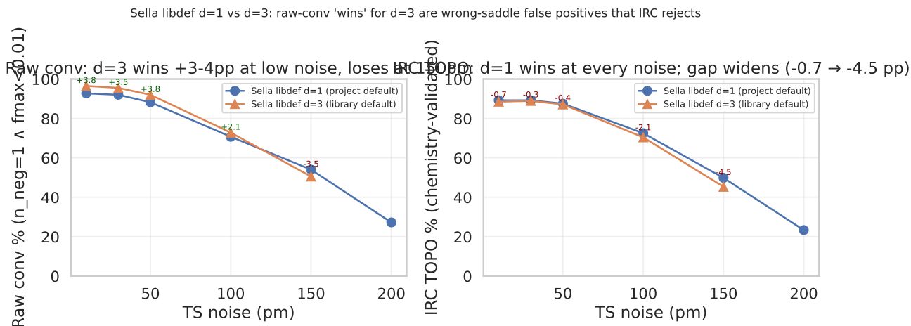
Figure 10: Sella Eckart Hess.Freq.=1 (d=1, project) vs Hess.Freq.=3 (d=3, library default) across noise. Left: TS conv (d=3 wins +3-4 pp at low noise; loses at 150 pm). Right: IRC TOPO (d=1 wins at every noise level; gap monotonically widens with noise from -0.7 pp at 10 pm to -4.5 pp at 150 pm). The d=3 raw-conv "wins" are wrong-saddle false positives that IRC catches and rejects. Source: runs/test_hessfreq/sella.cartack.libdef_d3/ + runs/irc.sella.libdef_d3/ , 200 pm cells pending (SLURM 60769799/60769872).
