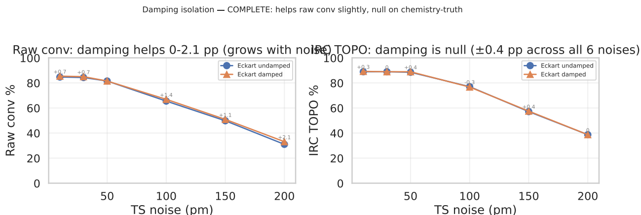
Figure 9: Damping helps raw conv slightly, null on chemistry. Left: damped Eckart eig-switch beats undamped by 0–2.1 pp on raw conv at every noise, with the benefit growing monotonically with noise. Right: damping is \pm 0.4 pp on IRC TOPO at every noise — null. Mechanism: damping ( |\lambda_i| floor at min_curvature ) prevents tiny eigenvalues from generating divergent Newton steps, which matters more at high noise where eigenvalues fluctuate. But it doesn’t change which basin the trajectory ends up in. Use damped — never hurts, helps a hair on raw conv.
