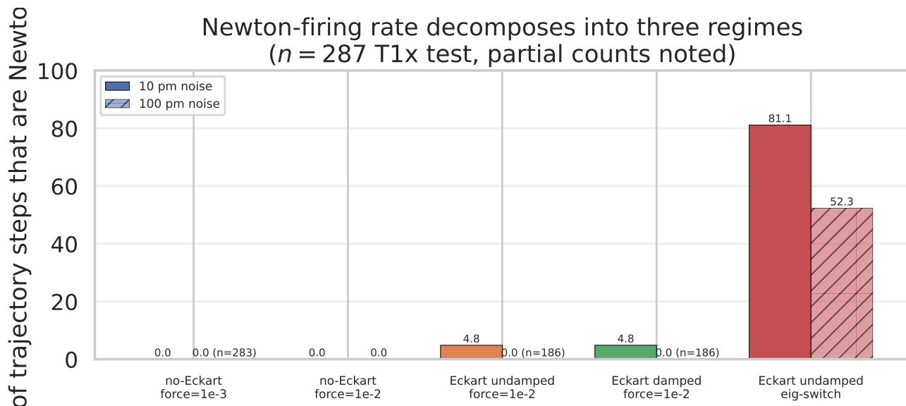
Figure 7: Three regimes of Newton activity. Per-step Newton fraction by config \times noise. (1) Never: no-Eckart with \text{sf} \leq 0.01 , Cartesian force-norm never crosses threshold. (2) Sometimes: Eckart force-switch \text{sf}=0.01 fires Newton 5% of steps at 10 pm, 0% at 100 pm. (3) Always: Eckart eigenvalue-switch fires Newton 52–81% of steps at all noise levels. Only eigenvalue-switch reaches Newton reliably at high noise.
