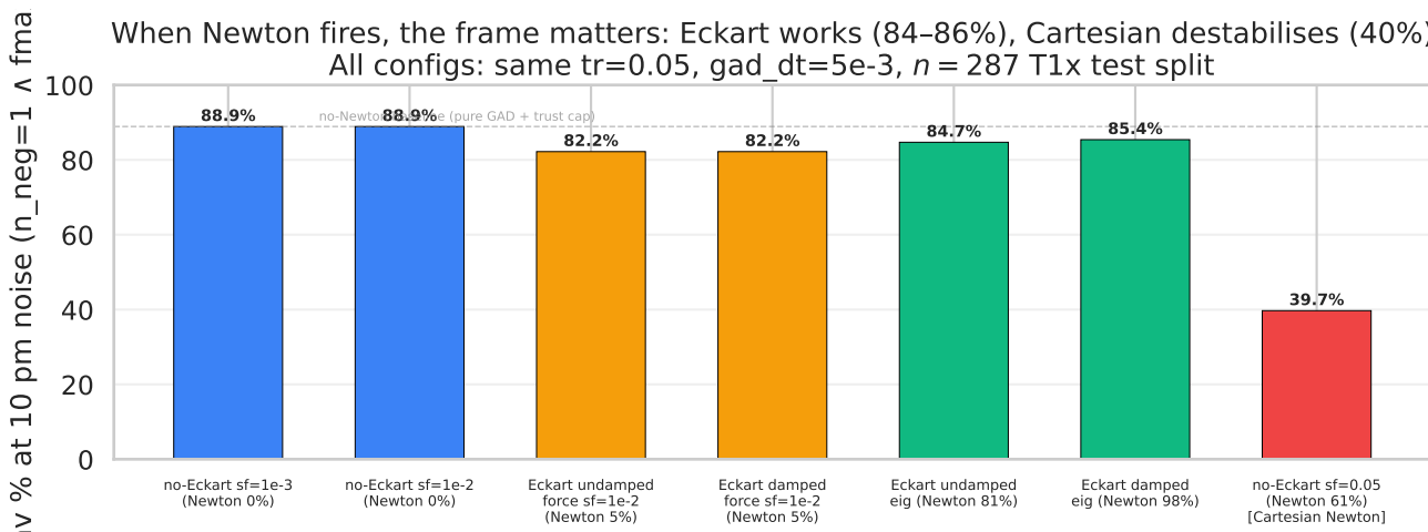
Figure 8: Frame matters when Newton fires. 7 configurations at 10 pm, color-coded by Newton-firing regime. Red bar = no-Eckart with sf=0.05 (Cartesian Newton fires 61% of steps) — raw conv crashes to 39.7%, but IRC TOPO is still 88.9% , tied with all other configs. Cartesian Newton displaces the geometry by 0.3–1 Å (RMSD- intended drops to 26% vs other configs’ 45–46%) but keeps the trajectory in the right basin. Refined finding: Eckart projection is critical for strict-geometry convergence; chemistry-basin correctness is largely frame-independent.
