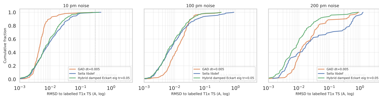
Figure 6: RMSD distributions of converged TSs vs the labelled T1x reference. CDFs across three noise levels ( n=287 each, converged samples only). At 10 pm all three families are tight ( \leq 0.05 Å). At 100 pm Sella develops a long right tail (some "converged" Sella TSs sit \sim 0.2 Å off); hybrid stays tight. At 200 pm the hybrid is dramatically tighter — the green curve rises sharply at low RMSD while Sella's blue and GAD's orange extend past 0.5 Å. The 0.3 Å threshold (dashed) is the RMSD-intended cutoff. Source: rmsd_distributions_2026-05-11.csv .
