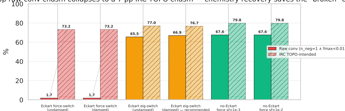
Figure 11: The 65 pp raw-conv chasm collapses to a 7 pp IRC TOPO chasm at 100 pm. Three tiers: (red) Eckart force-switch (Newton barely fires, 1.7% raw, +71.5 pp recovery); (orange) Eckart eig-switch (Newton fires often, mid recovery); (green) no-Eckart force-switch (GAD-with-trust-cap, high raw conv and TOPO). Convergence threshold strictness \neq chemistry basin correctness. A trajectory can stay in the right basin for 1000 steps without ever crossing f_{\max} < 0.01 .
