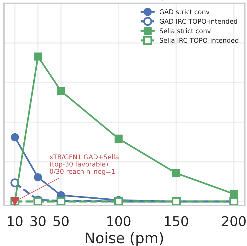
SCINE/DFTB0: GAD's IRC TOPO \geq Sella's at every noise level (+9.4pp at 10pm)
