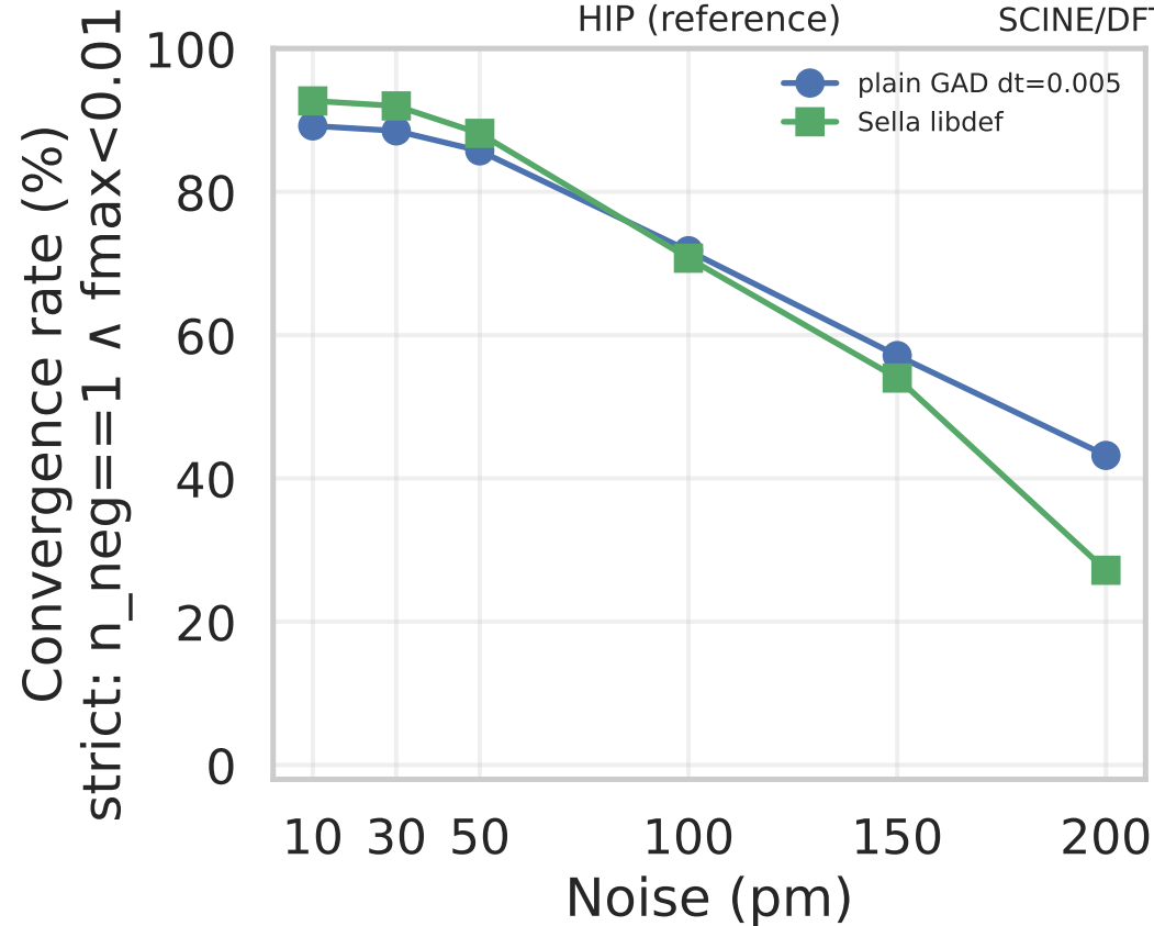
Noise sweep, T1x test (n=287): HIP reference vs SCINE/DFTB0 + xTB/GFN1
