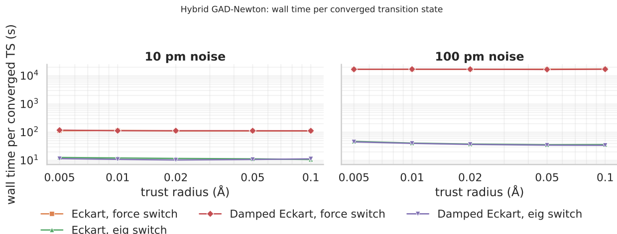
Figure 7: Wall-time per converged TS. The switch=False rows are two orders of magnitude slower than switch=True at 100pm (because the denominator n_{\text{conv}} is 1 vs \sim 190 ); at 10pm the gap is 10\times . switch=True saturates at \sim 10\text{s/conv} at 10pm and \sim 35\text{s/conv} at 100pm.
