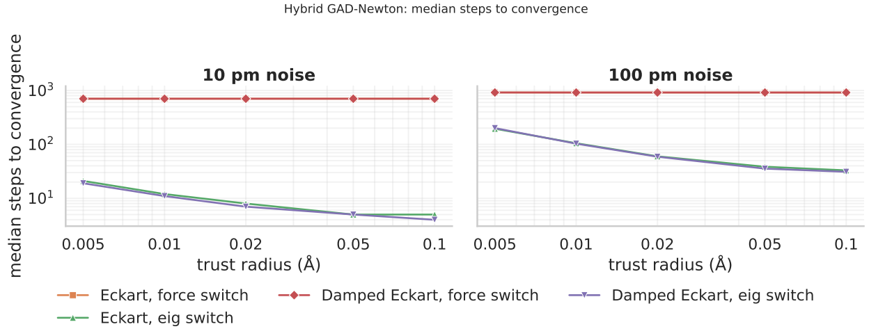
Figure 6: Median steps to converge as a function of trust radius. Y-axis log-scaled. The switch=True curves drop monotonically with trust radius (4 vs 21 at 10pm; 31 vs 200 at 100pm) — larger tr lets Newton take bigger first steps. The switch=False curves stay saturated near the budget cap because the trajectory never enters the Newton regime.
