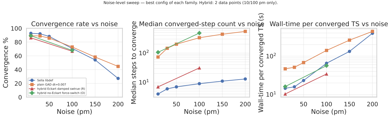
Figure 1: Best config of each family vs TS-noise level (10, 30, 50, 100, 150, 200 pm). Left: convergence %. Centre: median converged-step count (log y). Right: wall-time per converged TS (log y). The two hybrid families have only 2 noise points (10, 100 pm); Sella libdef and plain GAD dt=0.007 cover all 6. Source: analysis_2026_04.29/noise_sweep_unified.csv.
