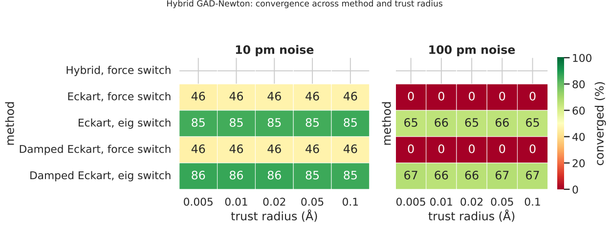
Figure 2: Conv % across the 4-method \times 5-trust-radius grid, per noise level. Each cell is one of the 40 jobs ( n = 287 test samples, \leq 1000 steps). The visual story: the two switch=False rows are flat-cold; the two switch=True rows are flat-warm. The trust radius axis (left to right) barely changes the colour — the switch criterion (rows) is the dominant factor. Reference: vanilla GAD dt=0.005 gets \sim 89/72\% at the corresponding noise.
