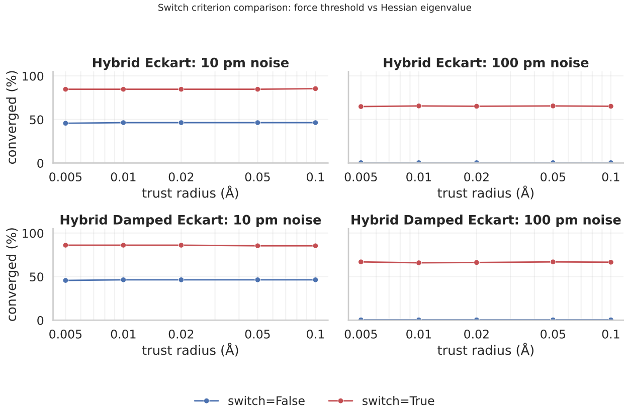
Figure 4: For both Eckart families (top: hybrid_eckart ; bottom: hybrid_damped_eckart ): switch=False vs switch=True curves side-by-side. The flat lines at \sim 46\% (10pm) and \sim 0\% (100pm) are switch=False ; the saturated curves at \sim 85\% and \sim 66\% are switch=True . Damping (lower row) gives a slight upward shift at every tr.
