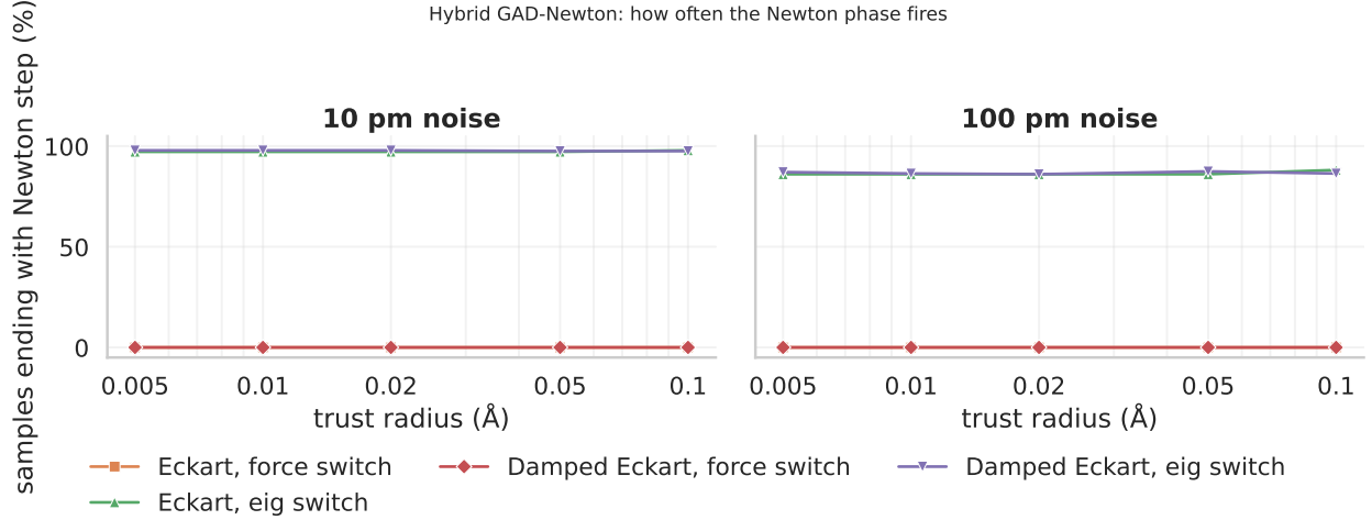
Figure 5: Fraction of samples whose terminating step used the Newton phase (vs GAD). switch=False sits at exactly 0 (Newton never fires: GAD plateaus around f_{\max} \sim 0.01 and never crosses \|F\| < 10^{-3} ). switch=True sits at 0.86–0.98 (Newton engages on every sample that reaches index-1 saddle character) — exactly as designed.
