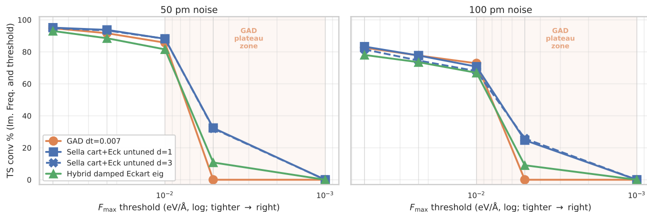
Figure 8: The f_{\max} plateau, hypothesis confirmed. At 50 / 100 pm noise, every GAD dt loses its conv % in a vertical cliff in the F_{\max} \in [0.001, 0.01] band — the “GAD plateau zone” (orange shading). Sella’s Newton step retains 24–34% at F_{\max} < 0.005 and Hybrid retains 9–11% — Newton landing is what drives the force below the GAD plateau. None of the three reach F_{\max} < 0.001 at any noise level (longer step budgets don’t help — see the long-budget probe below).
