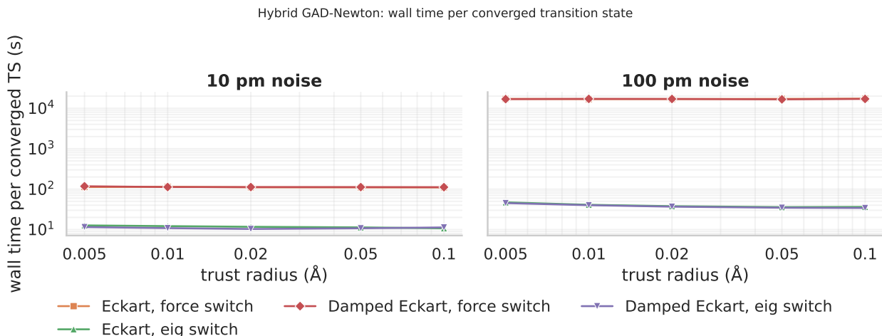
Figure 6: Wall-time per converged TS. The switch=False rows are two orders of magnitude slower than switch=True at 100pm (because the denominator n_{\text{conv}} is 1 vs \sim 190 ); at 10pm the gap is 10\times . switch=True saturates at \sim 10\text{s/conv} at 10pm and \sim 35\text{s/conv} at 100pm.
