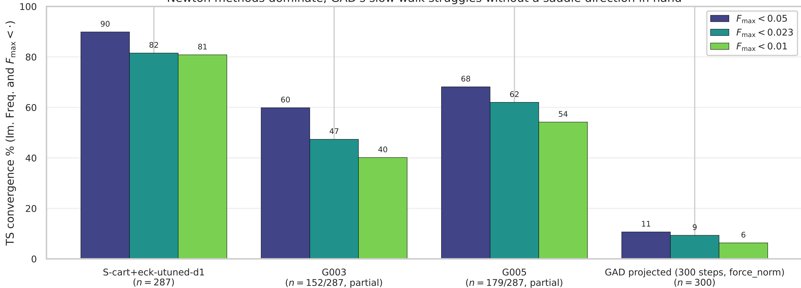
Starting from REACTANT @ 0 pm noise (T1x test split) Newton methods dominate; GAD's slow walk struggles without a saddle direction in hand
