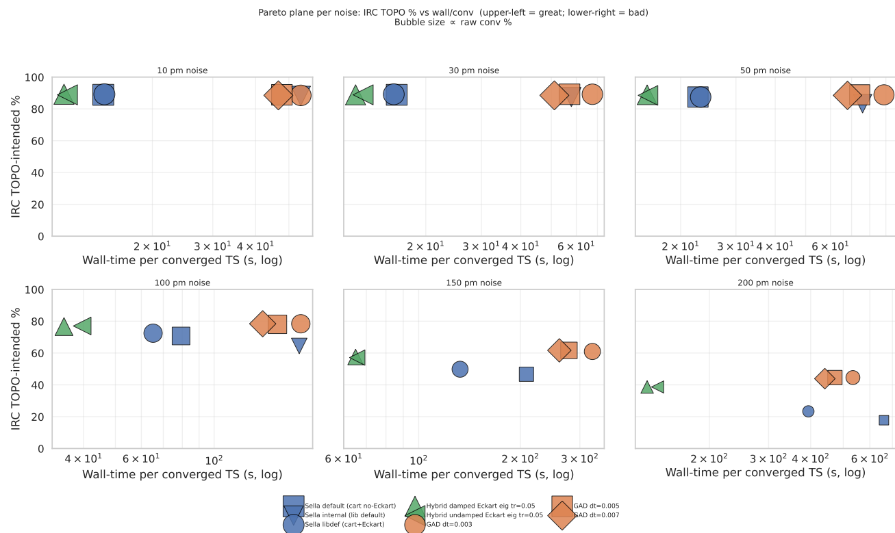
Figure 2: Pareto plane per noise. x = wall-time per converged TS (log); y = IRC TOPO. Bubble size \propto raw conv. Upper-left = great (fast AND chemistry-correct); lower-right = bad (slow AND chemistry-failing). Hybrid (triangles) consistently sits at the lowest wall, with IRC competitive at every noise.
