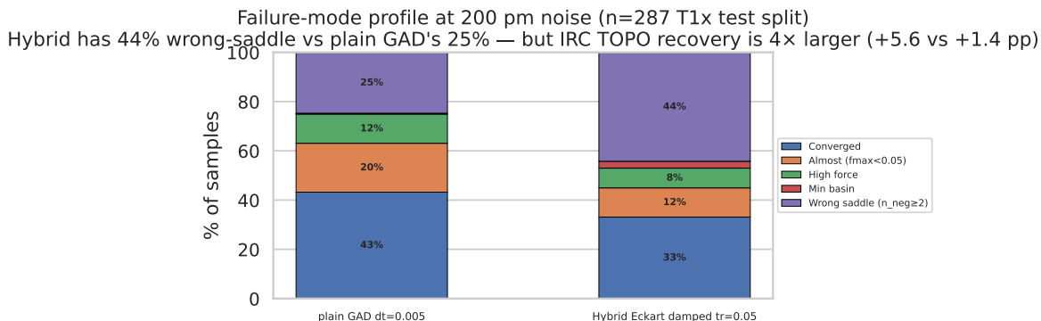
Figure 5: Failure-mode profile at 200 pm. Hybrid pays a wrong-saddle penalty (44% vs plain GAD’s 25%) when Newton’s eigenvector-following lands on the wrong mode. But many of those wrong-saddle geometries are still in the right reaction basin, so IRC recovers them. Result: hybrid trails plain GAD by 6 pp on IRC TOPO at 200 pm, not 19 pp as raw saddle character suggests.
