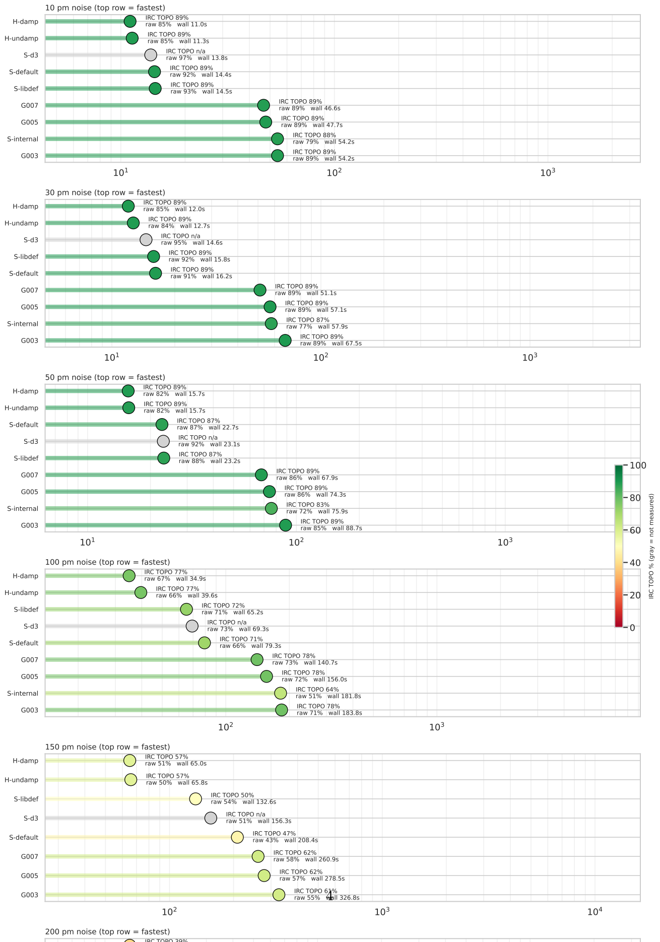
Method rankings by wall-time per converged TS • head color = IRC TOPO
