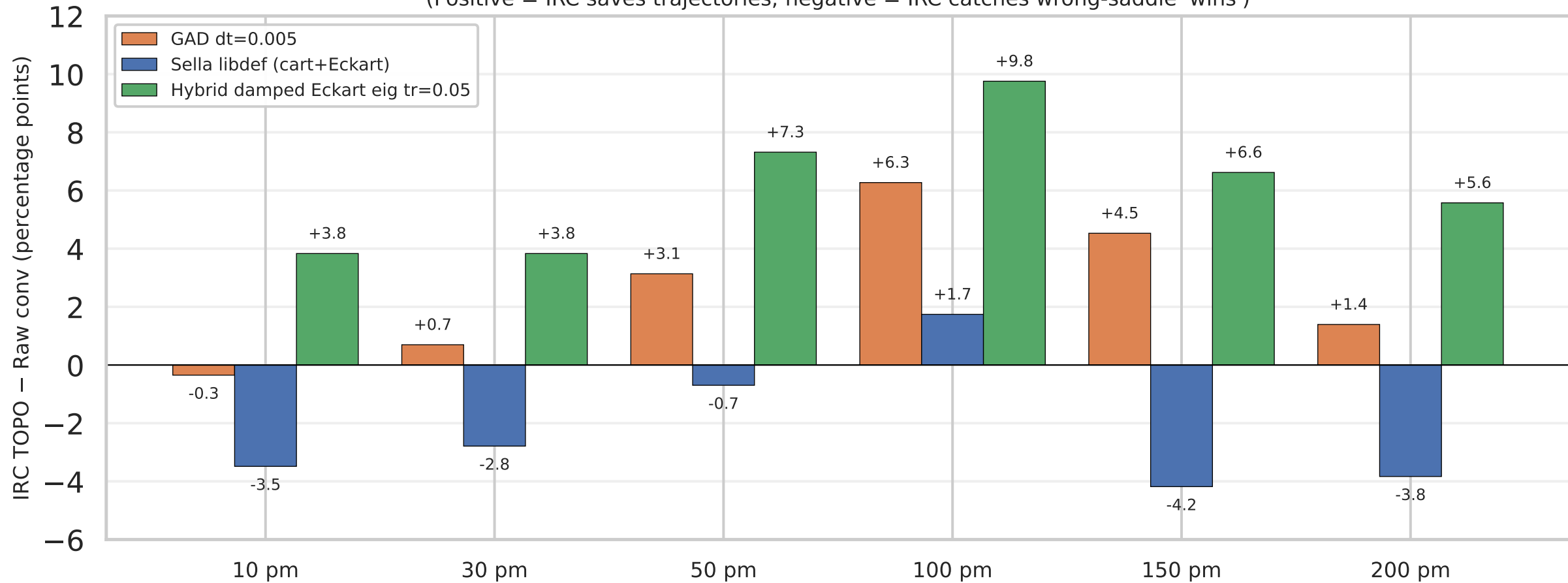
Who gains from IRC chemistry validation? (Positive = IRC saves trajectories; negative = IRC catches wrong-saddle 'wins')
