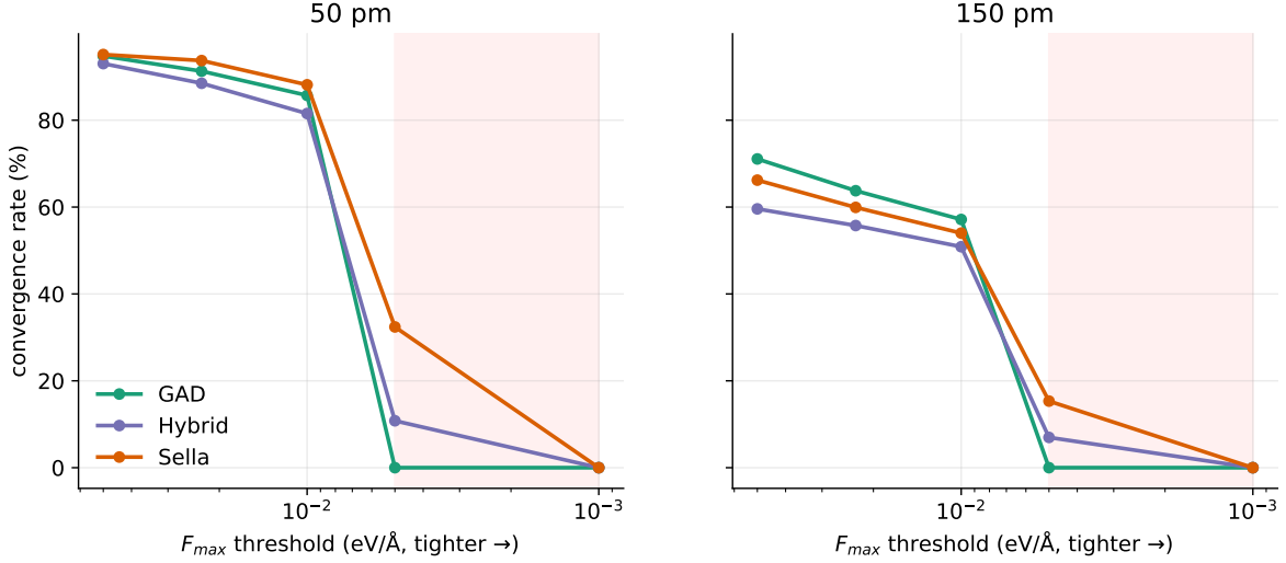
Figure 8: The F_{\max} plateau (convergence vs. threshold; tighter to the right). GAD drops vertically near 0.01; Sella and the hybrid descend into 0.005 via Newton landing.
