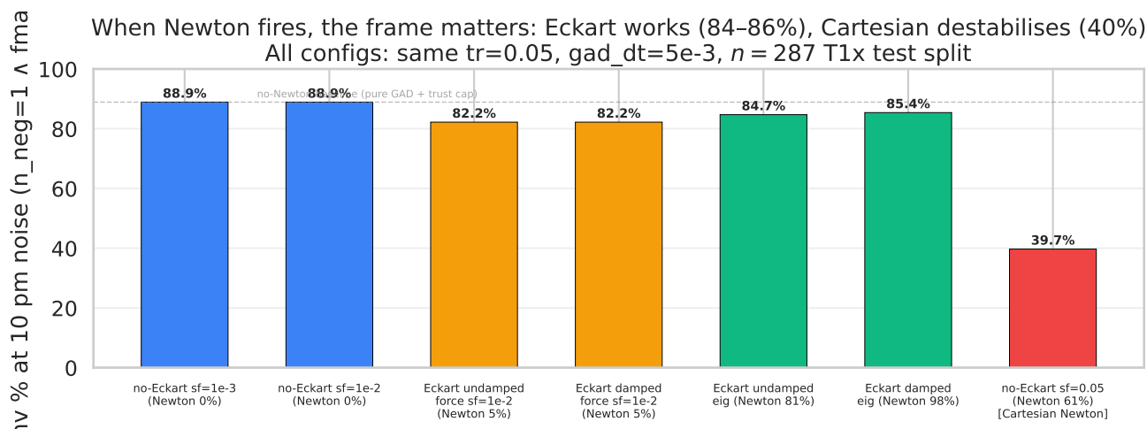
Figure 9: Frame matters when Newton fires. 7 configurations at 10 pm, color-coded by Newton-firing regime. Red bar = no-Eckart with sf=0.05 (Cartesian Newton fires 61% of steps) — raw conv crashes to 39.7%, but IRC TOPO is still 88.9% , tied with all other configs. Cartesian Newton displaces the geometry by 0.3–1 Å (RMSD- intended drops to 26% vs other configs’ 45–46%) but keeps the trajectory in the right basin. Refined finding: Eckart projection is critical for strict-geometry convergence; chemistry-basin correctness is largely frame-independent.
