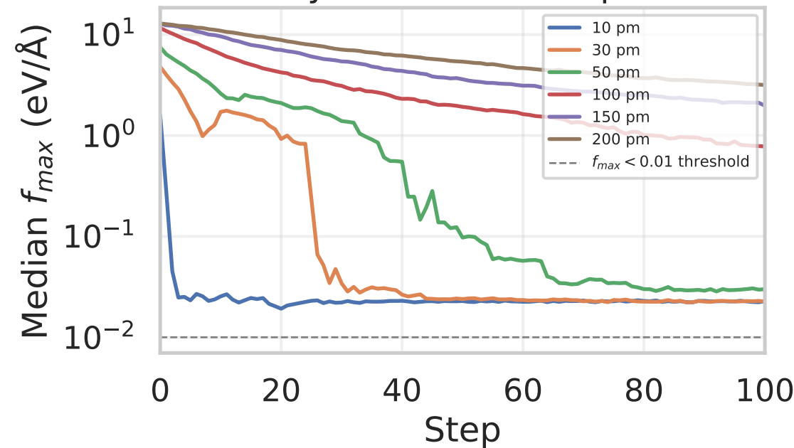
Force descent — hybrid Eckart damped swtrue tr=0.05
