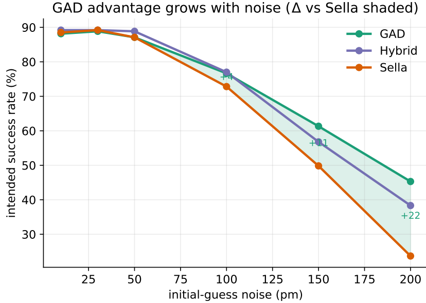
Figure 2: IRC convergence for all three methods; the GAD–Sella gap is shaded. Paired-McNemar (GAD vs. Sella): indistinguishable \leq 50 pm ( p=1.0 ), emerging at 100 pm ( p=0.10 ), highly significant at 150 pm ( p=3.8 \times 10^{-5} ) and 200 pm ( p=1.7 \times 10^{-13} ).
