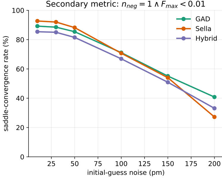
Figure 7: Secondary metric: F_{\max}/n_{\text{neg}} convergence rate ( n_{\text{neg}}=1 \wedge F_{\max}<0.01 ) vs. noise, n = 287 . Sella leads at low noise; GAD overtakes at high noise — but convergence is not chemistry (cf. Fig. 1).
