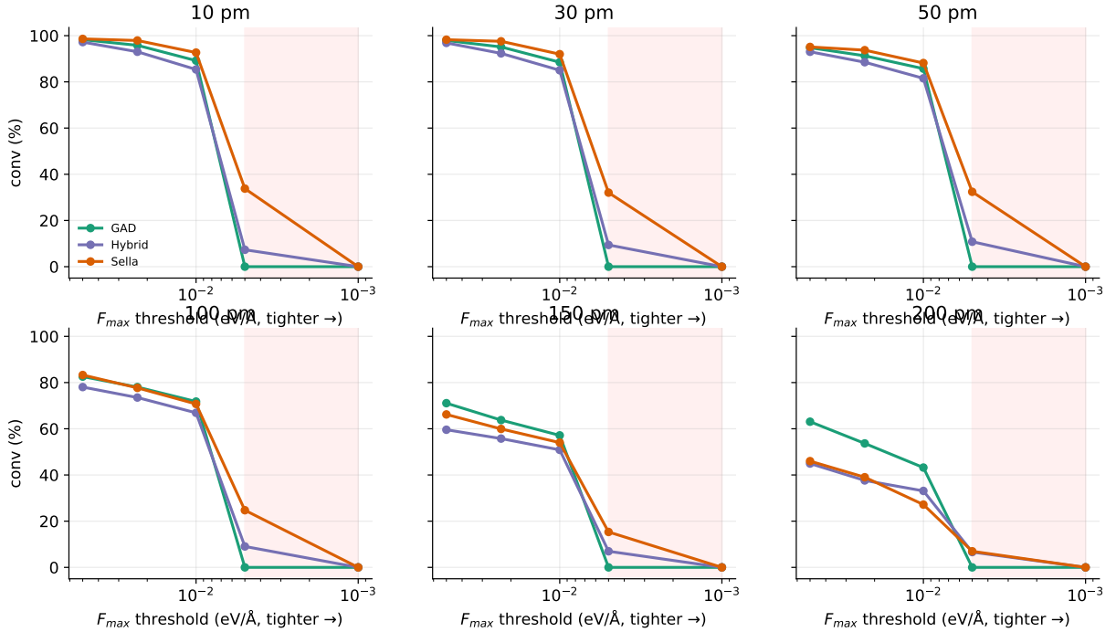
Figure 9: F_{\max}/n_{\text{neg}} convergence vs. F_{\max} threshold, one panel per noise level (10–200 pm). Each panel plots convergence rate (%) against the force threshold (log x , tightening to the right; shaded = plateau zone) for GAD, the hybrid, and the Sella baseline. The GAD curve collapses vertically to 0% at F_{\max} < 0.005 in every panel, whereas Sella and the hybrid descend further — the plateau is a property of the fixed-step first-order dynamics, universal across noise.
