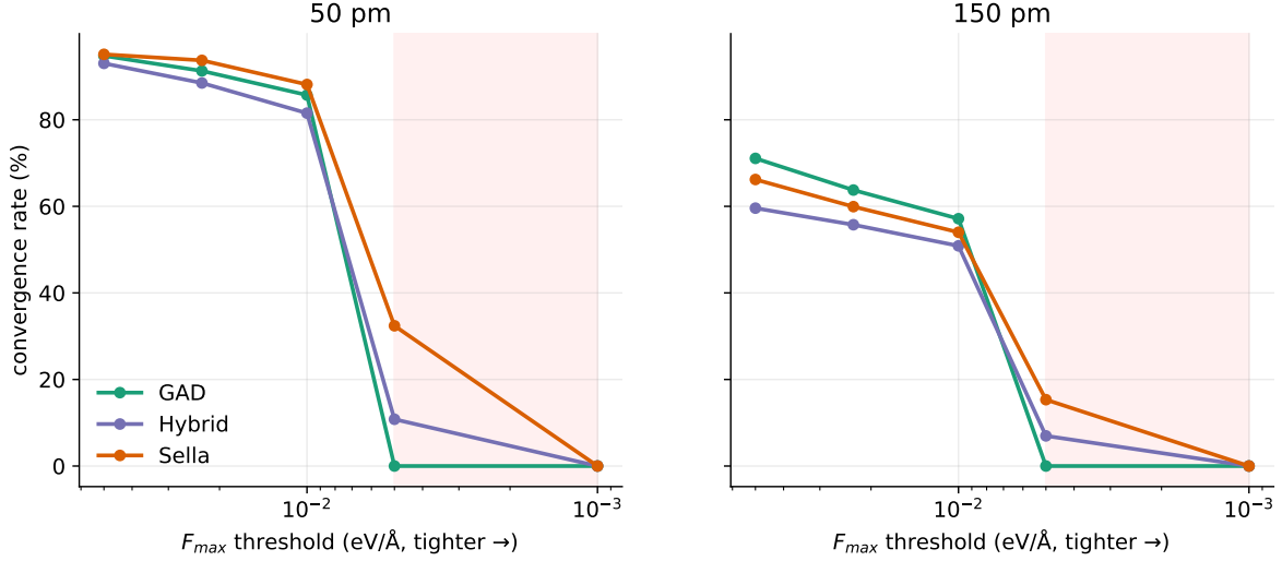
Figure 8: The F_{\max} plateau (50 and 150 pm noise). F_{\max}/n_{\text{neg}} convergence rate (%), vs. the F_{\max} threshold ( x , log axis, tightening to the right; shaded = the sub-0.005 plateau zone), one line per method. GAD drops vertically near F_{\max}=0.01 — it has essentially no converged samples below it — whereas Sella and the hybrid keep descending into the 0.005 band because their trust-radius-capped Newton step continues to drive the residual force down. No method reaches 0.001 within the 2,000-step budget.
