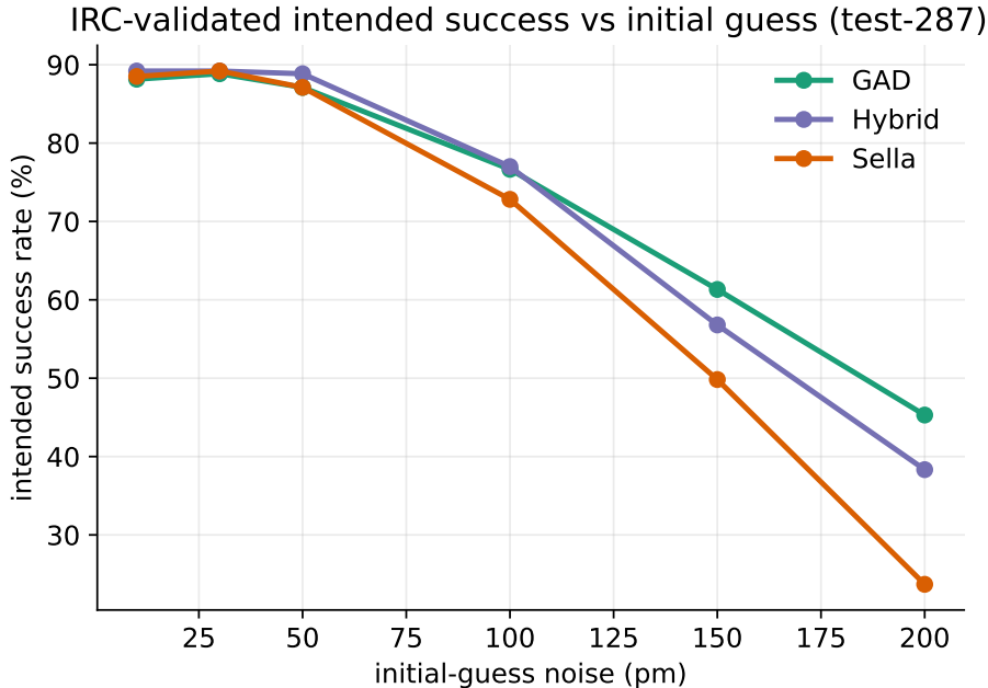
Figure 1: Primary metric: IRC convergence rate vs. initial-guess noise, n = 287 . x-axis : isotropic Gaussian perturbation of the true saddle (10–200 pm). y-axis : % of the 287 reactions whose forward and backward IRC graph-match both the intended reactant and product. One line each for GAD, the hybrid, and the strongest Sella baseline. The three methods coincide while the guess is good; GAD and the hybrid retain far more intended reactions as it degrades. ( F_{\max}/n_{\text{neg}} convergence is shown separately in Fig. 7.)
