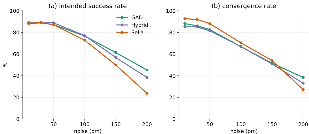
Figure 14: Primary result (focused). Intended-reaction success (left) and F_{\max}/n_{\text{neg}} convergence (right) vs. noise for GAD, the hybrid, and the strongest Sella baseline. The methods tie when the guess is good and GAD pulls ahead as it degrades; the crossover holds on both axes.
