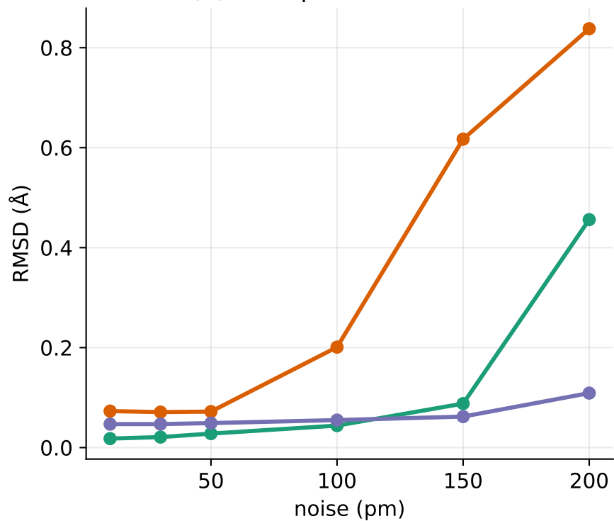
(b) 95th-percentile RMSD
