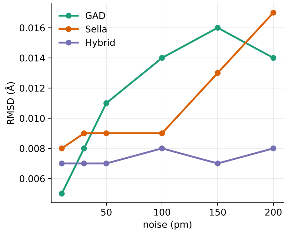
(a) median RMSD to true TS
