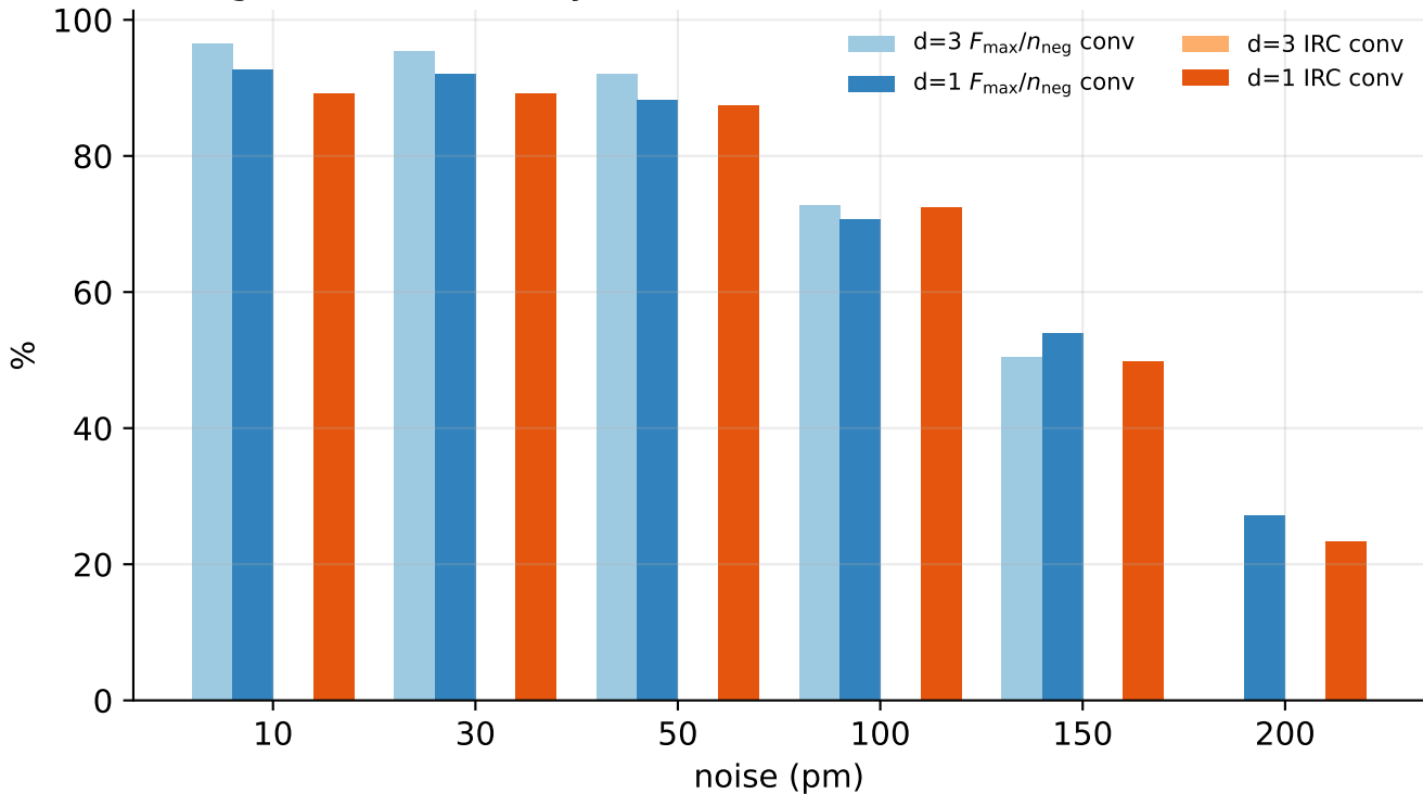
Convergence \neq chemistry: d=3 has more F/n conv, d=1 more IRC conv
