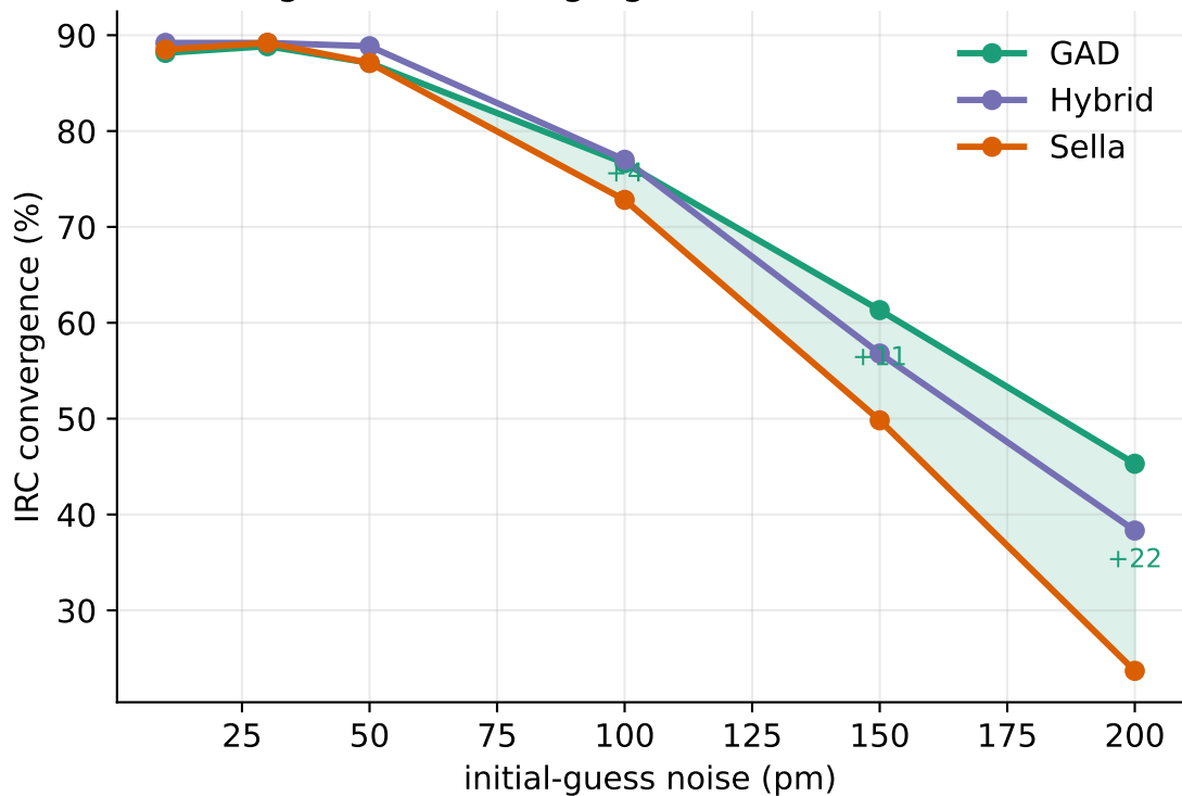
GAD IRC-convergence advantage grows with noise ( \Delta vs Sella shaded)
