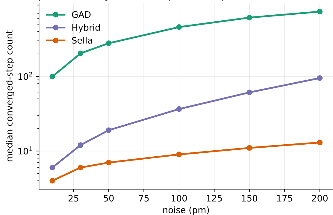
Steps to convergence (cheap GAD steps vs few Newton steps)
