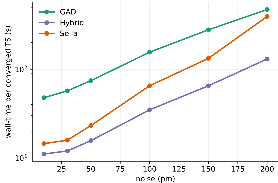
Cost: wall-time per converged TS
