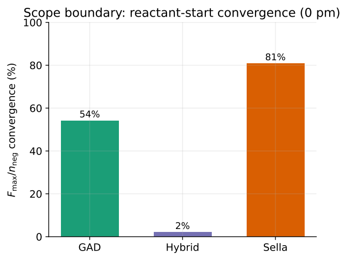
Figure 20: Scope boundary. From a reactant start the GAD family is weak and Sella wins; GAD needs a near-saddle guess for the reaction mode to be identifiable.
