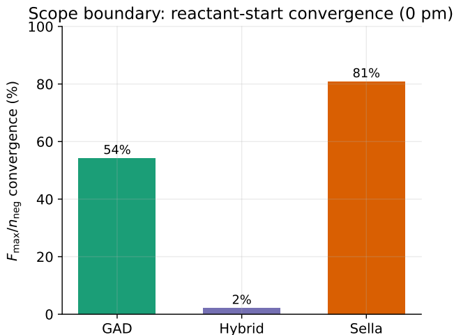
Figure 12: Scope boundary. Convergence from a reactant start: Sella wins; the GAD family needs a near-saddle guess.
