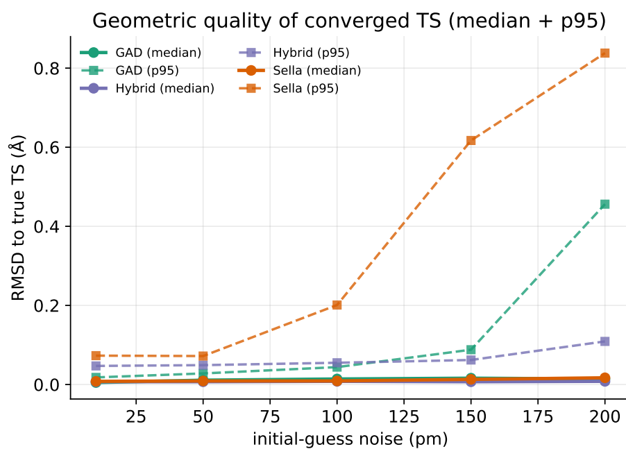
Figure 18: Geometric quality. Median and 95th-percentile RMSD of the converged TS to the labelled saddle vs. noise; the hybrid stays tight where Sella develops a large-RMSD tail.
