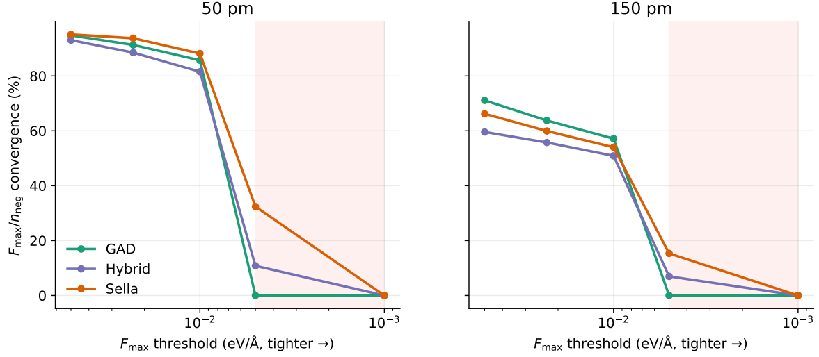
Figure 8: The F_{\max} plateau (50 and 150 pm noise). F_{\max}/n_{\text{neg}} convergence rate (% , y ) vs. the F_{\max} threshold ( x , log axis, tightening to the right; shaded = the sub-0.005 plateau zone), one line per method. GAD drops vertically near F_{\max}=0.01 — it has essentially no converged samples below it — whereas Sella and the hybrid keep descending into the 0.005 band because their trust-radius-capped Newton step continues to drive the residual force down. No method reaches 0.001 within the 2,000-step budget.
