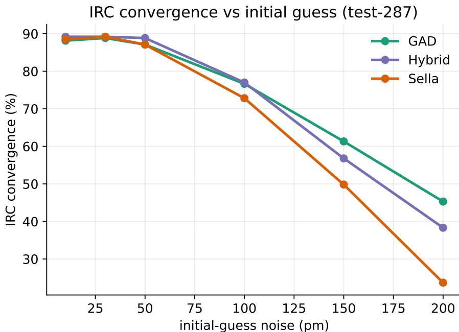
Figure 1: Primary metric: IRC convergence rate vs. initial-guess noise , n = 287 . x-axis : isotropic Gaussian perturbation of the true saddle (10–200 pm). y-axis : % of the 287 reactions whose forward and backward IRC graph-match both the intended reactant and product. One line each for GAD, the hybrid, and the strongest Sella baseline. The three methods coincide while the guess is good; GAD and the hybrid retain far more intended reactions as it degrades. ( F_{\max}/n_{\text{neg}} convergence is shown separately in Fig. 7.)
