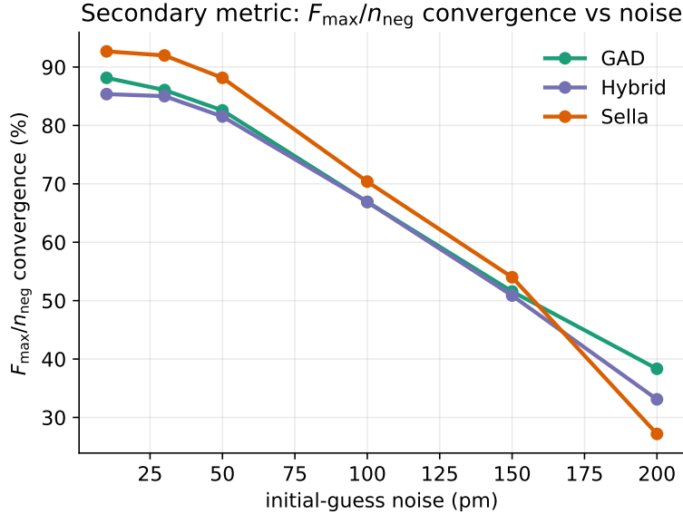
Figure 7: Secondary metric: F_{\max}/n_{\text{neg}} convergence rate ( n_{\text{neg}}=1 \wedge F_{\max}<0.01 ) vs. noise, n = 287 . Sella leads at low noise; GAD overtakes at high noise — but convergence is not chemistry (cf. Fig. 1).
