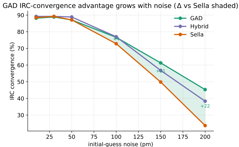
Figure 2: IRC convergence for all three methods; the GAD–Sella gap is shaded. Paired-McNemar (GAD vs. Sella): indistinguishable \leq 50 pm ( p=1.0 ), emerging at 100 pm ( p=0.10 ), highly significant at 150 pm ( p=3.8 \times 10^{-5} ) and 200 pm ( p=1.7 \times 10^{-13} ).
