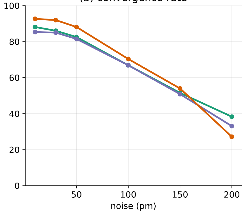
(b) convergence rate
