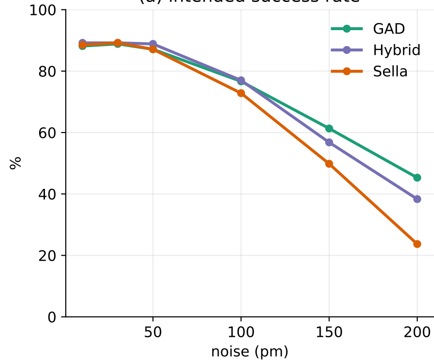
(a) intended success rate
