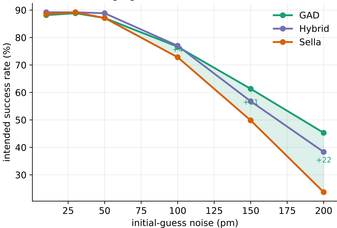
GAD advantage grows with noise ( \Delta vs Sella shaded)
