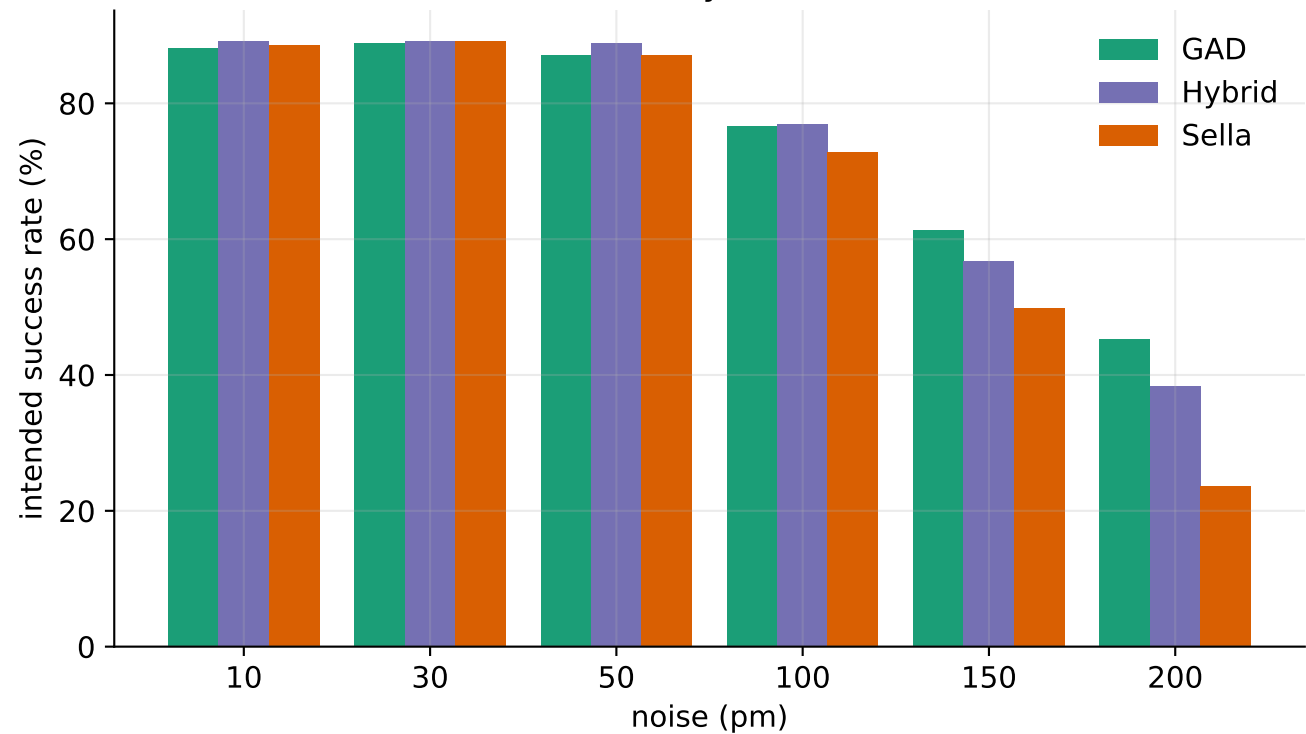
Intended success by method and noise
