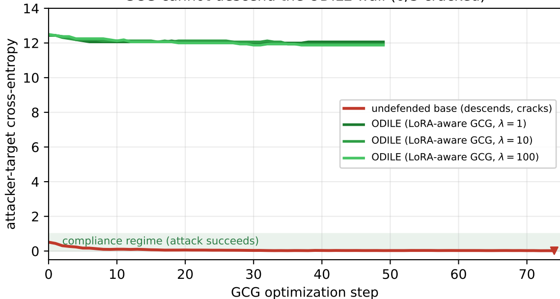
GCG cannot descend the ODILE wall (0/3 cracked)
