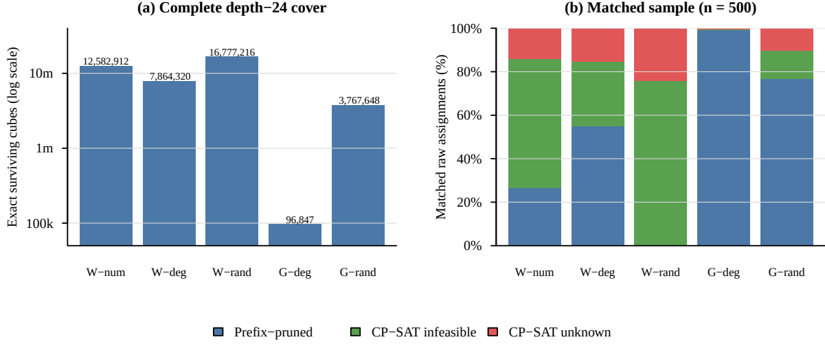
FIGURE 2. Split-policy ablation. Panel (a) gives the exact number of depth-24 cubes that survive AP-prefix pruning. Panel (b) gives outcomes on the same 500 uniformly sampled raw assignments for every policy. Prefix pruning is a sound closure; red segments are unresolved after the 60-s CP-SAT cap. Global degree sharply reduces the complete cover, while its rare survivors require a separate conquer-cost measurement. W and G abbreviate witness-restricted and global policies, respectively.
