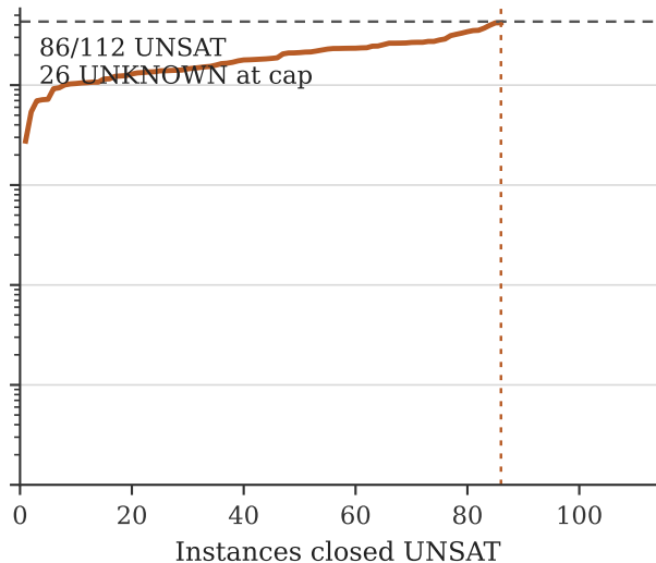
(b) CaDiCaL 3.0.0 on kissat residual
