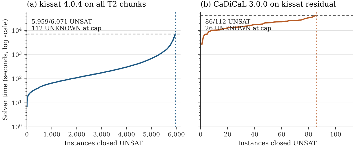
FIGURE 3. Cactus plots for the two-stage full-T2 portfolio. Curves contain only UNSAT rows; horizontal dashed lines mark each arm’s wall cap, and vertical dashed lines mark the number closed. Panel (b) is conditioned on the 112 kissat residuals and is therefore not a common-sample solver comparison.
