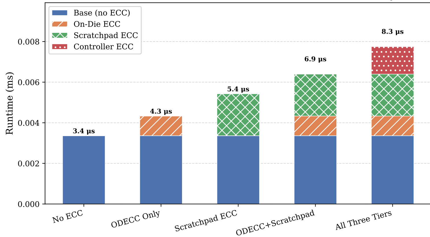
Fig 1 — PIMEval ADD_SCALAR Runtime per ECC Tier Configuration (256 INT32 elements, BitSIMD-V, 1 rank \times 1 bank \times 4 subarrays)
