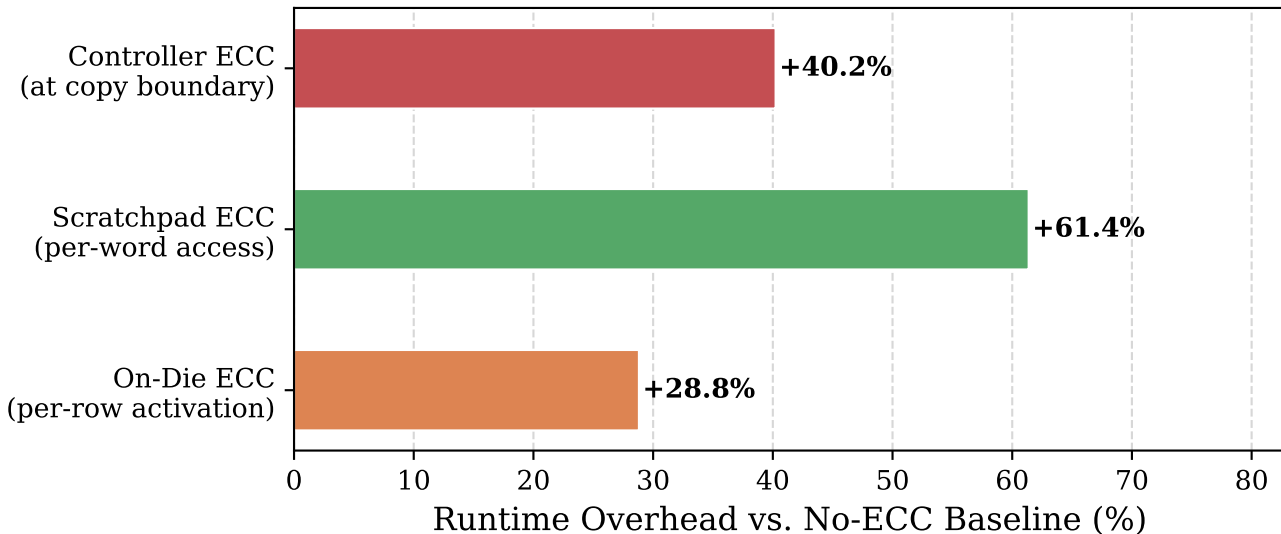
Fig 2 — Per-Tier ECC Runtime Overhead (marginal cost of enabling each tier independently)
