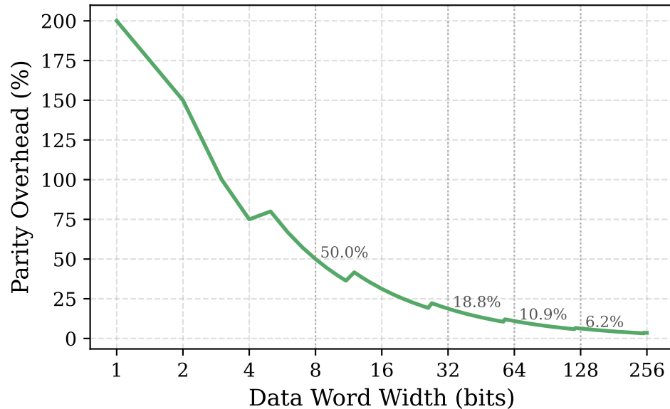
SECDED Storage Overhead %
