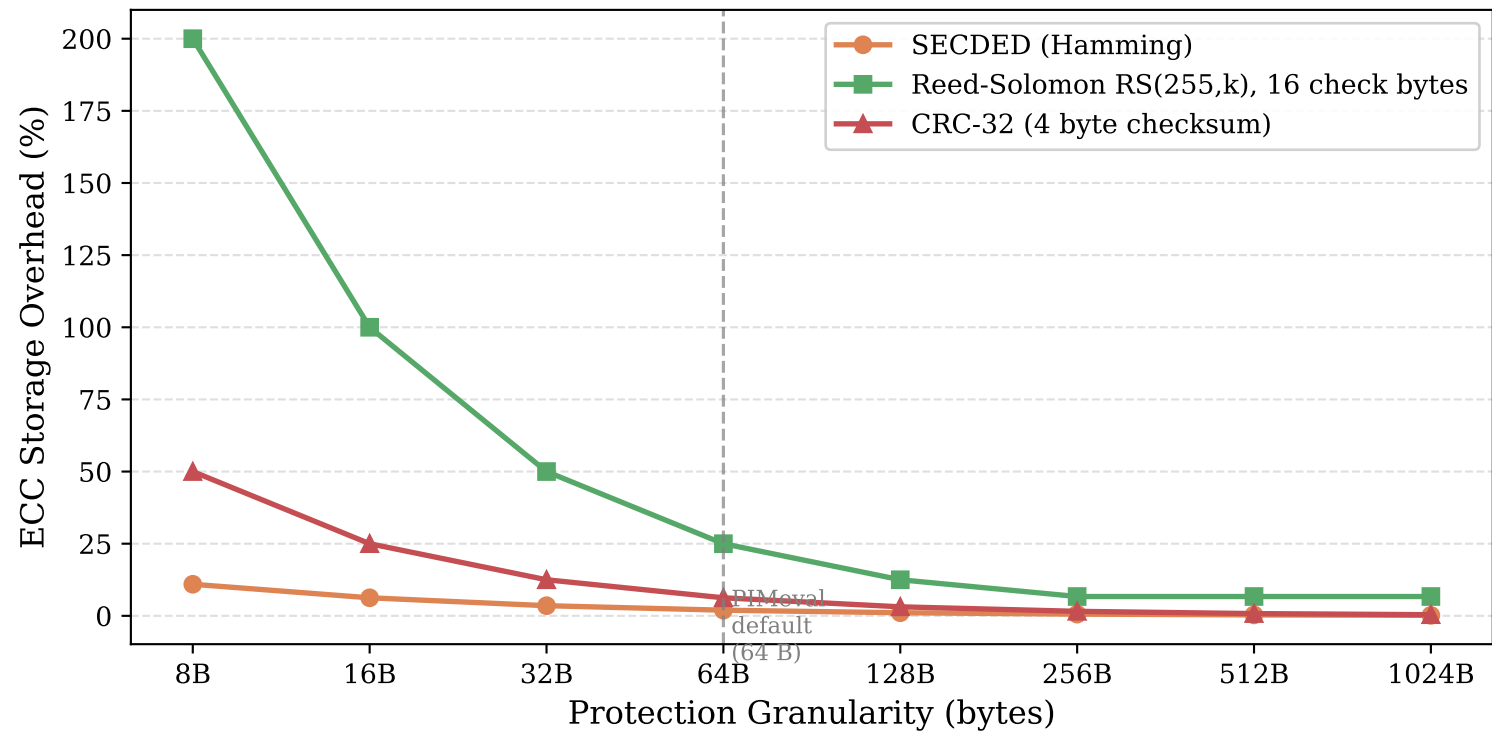
Fig 4 — Analytical ECC Storage Overhead vs. Protection Granularity (controller-tier codes: SECDED, Reed-Solomon, CRC-32)
