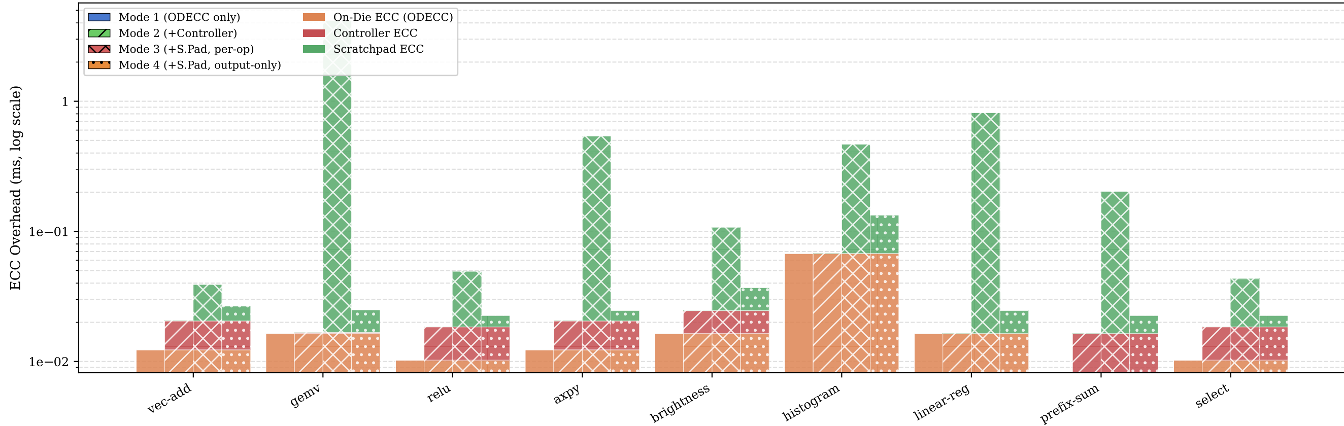
ECC Overhead by Tier and Mode — 9 Workloads × 4 Configurations (BITSIMD-V analytical, DDR5 baseline, 8192 INT32 elements)
