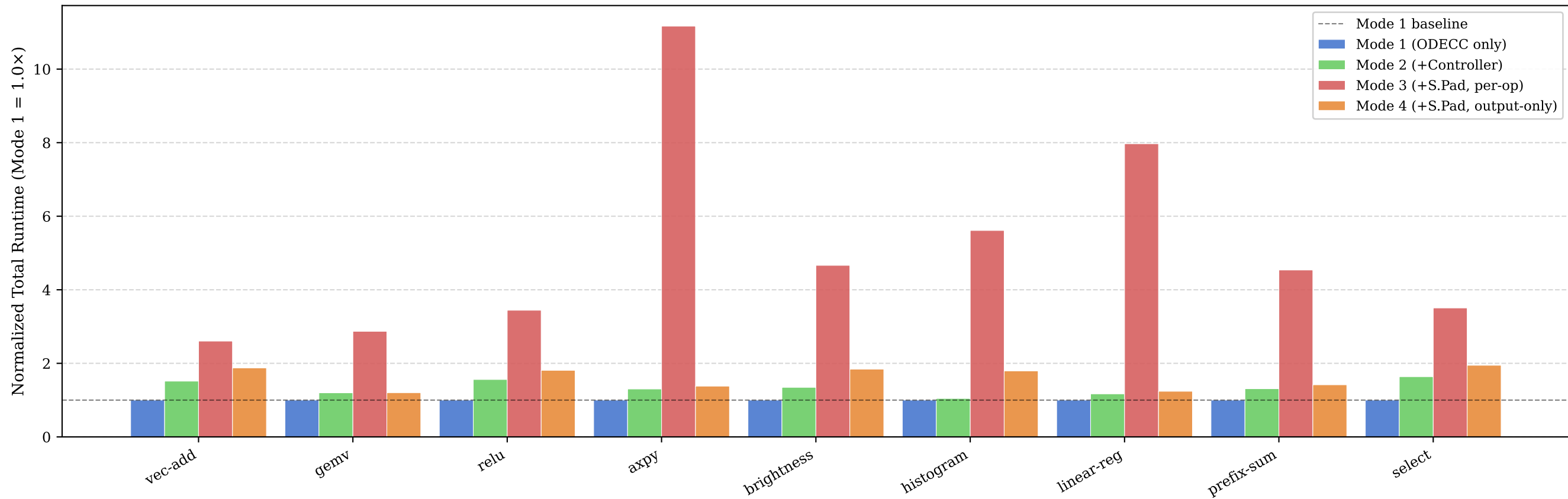
Total Runtime Normalized to Mode 1 Baseline Four ECC configurations — BITSIMD-V analytical, DDR5; Mode 4 = output-only scratchpad ECC
