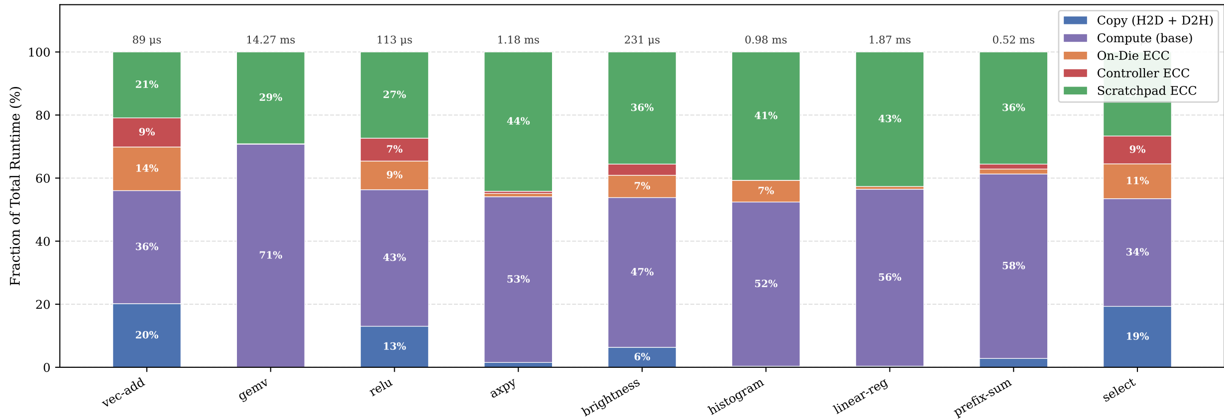
Mode 3 Runtime Breakdown per Tier (Conservative Scratchpad ECC, per-op) Absolute totals shown above bars — BITSIMD-V analytical, DDR5
